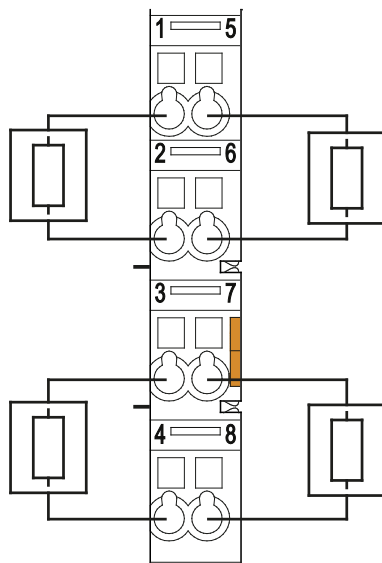
Figure 11: Connecting Diagram
