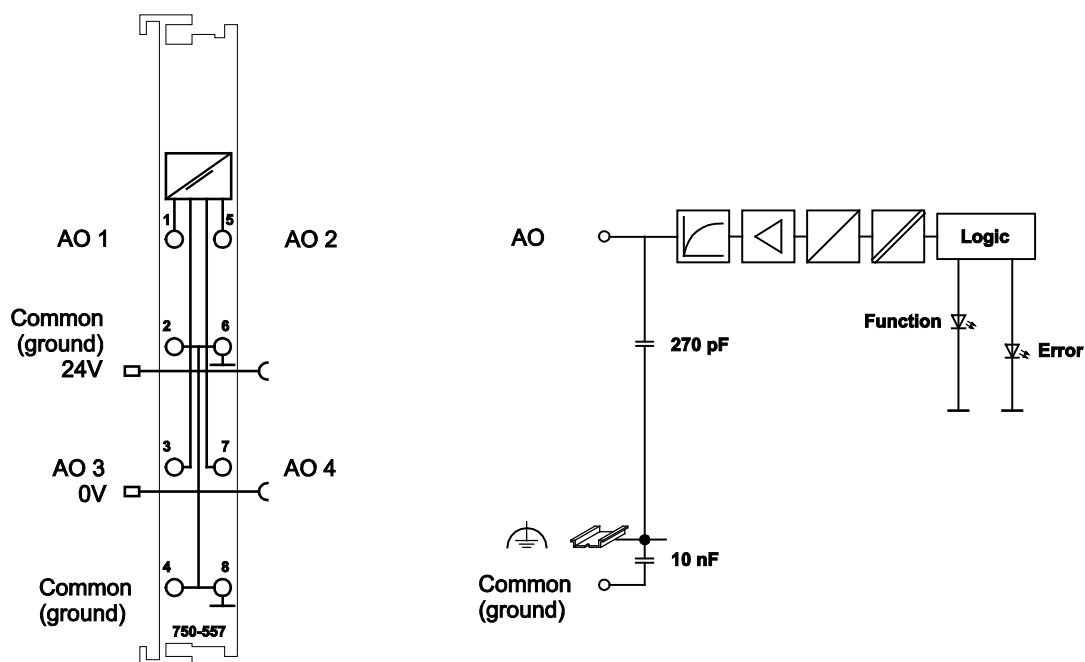
Figure 6: Schematic Diagram
