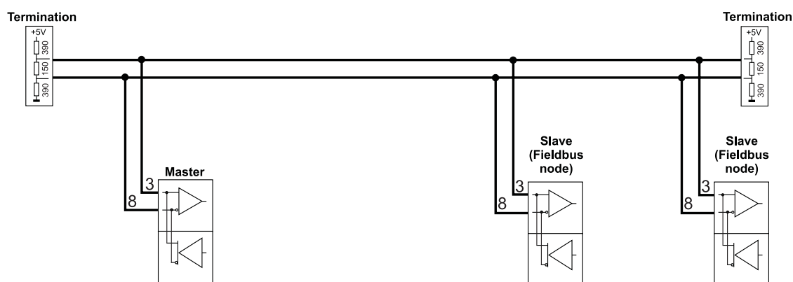
Fig. 2.7: 2 wire connection
