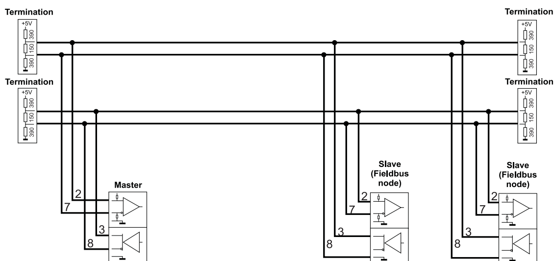
Fig. 2.8: 4 wire connection
