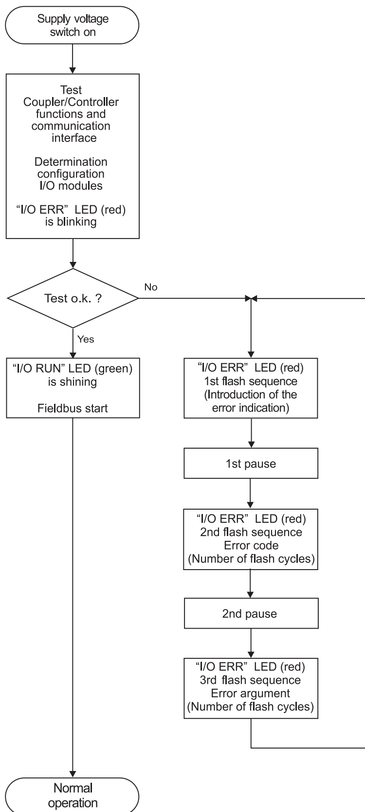
Fig. 6.2: Run-up coupler/controller
