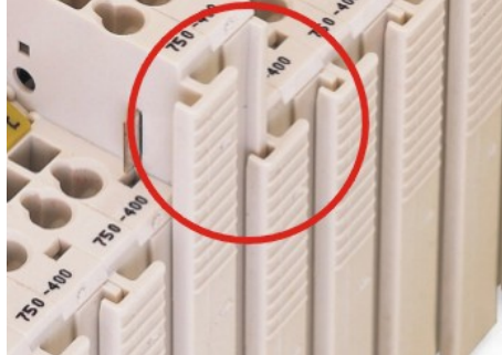
Figure 32: Insert I/O Module (Example)
