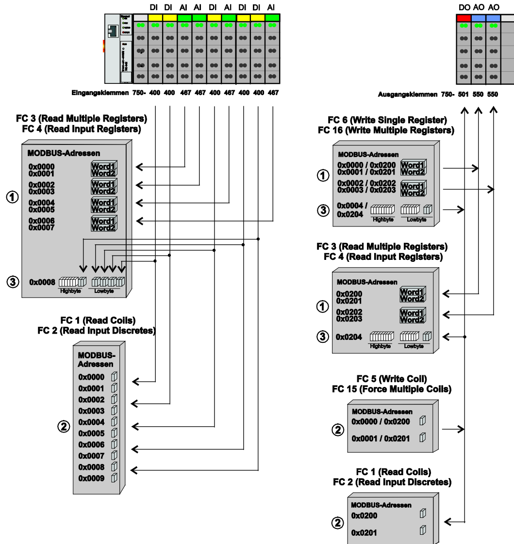
Figure 46: Using MODBUS Functions for a Fieldbus Coupler/Controller
