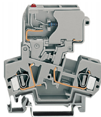
Figure 14: Fuse Modules with Pivotal Fuse Carrier, Series 281
