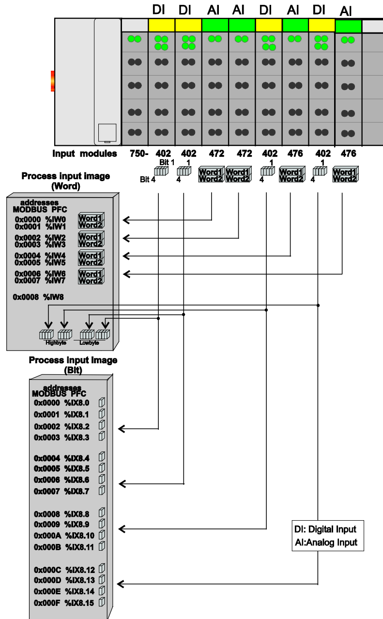
Figure 39: Example of an Input Process Image
