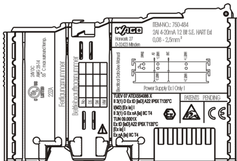
Figure 49: Side Marking Example for Ex i and IEC Ex i Approved I/O Modules According to CENELEC and IEC
