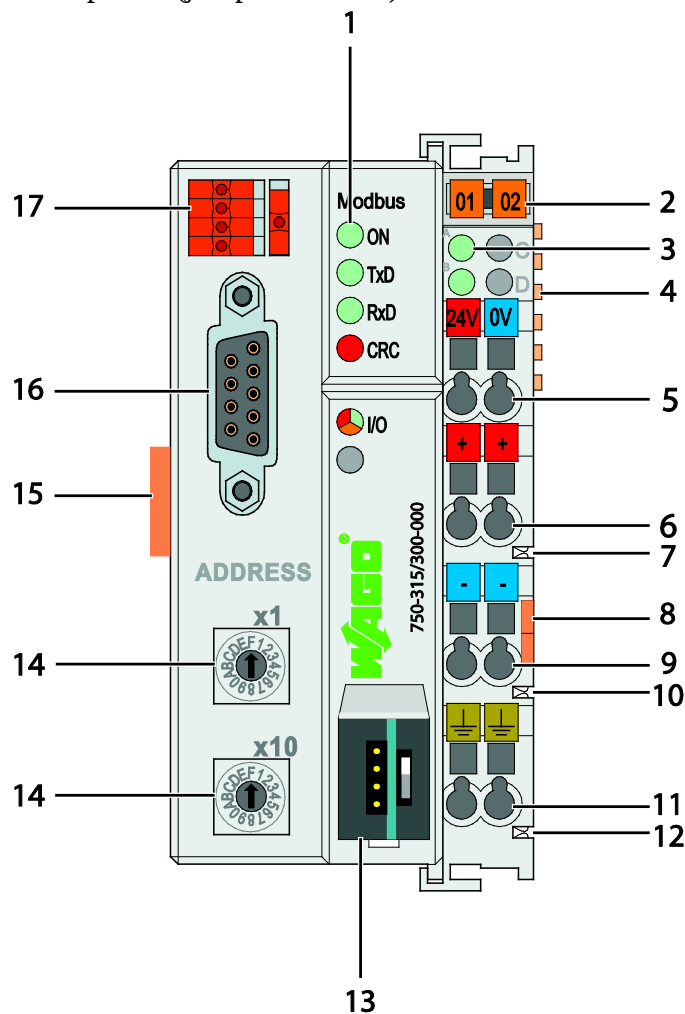
Figure 21: View MODBUS RTU Fieldbus Coupler
