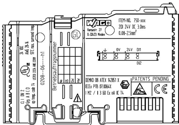
Figure 47: Side Marking Example for ATEX and IEC Ex Approved I/O Modules According to CENELEC and IEC
