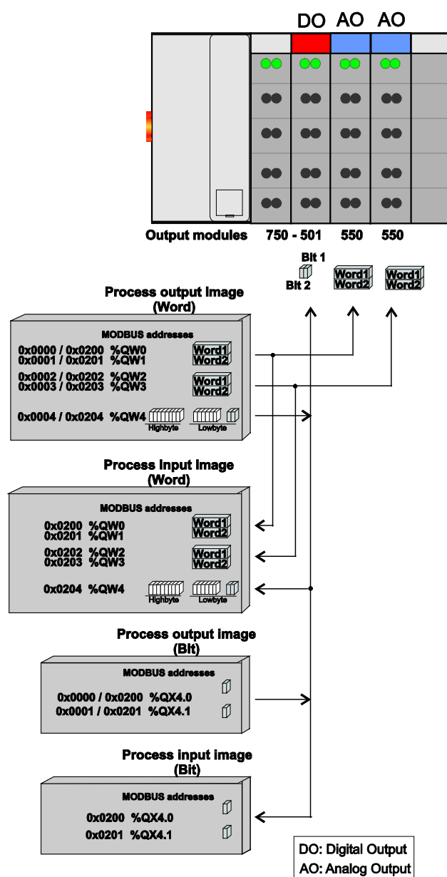
Figure 40: Example of an Output Image
