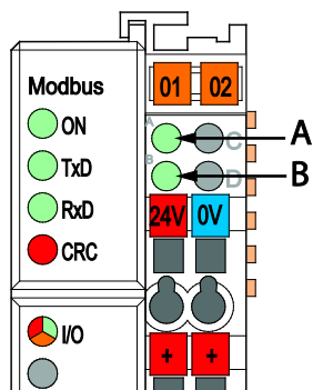
Figure 43: Display Elements
