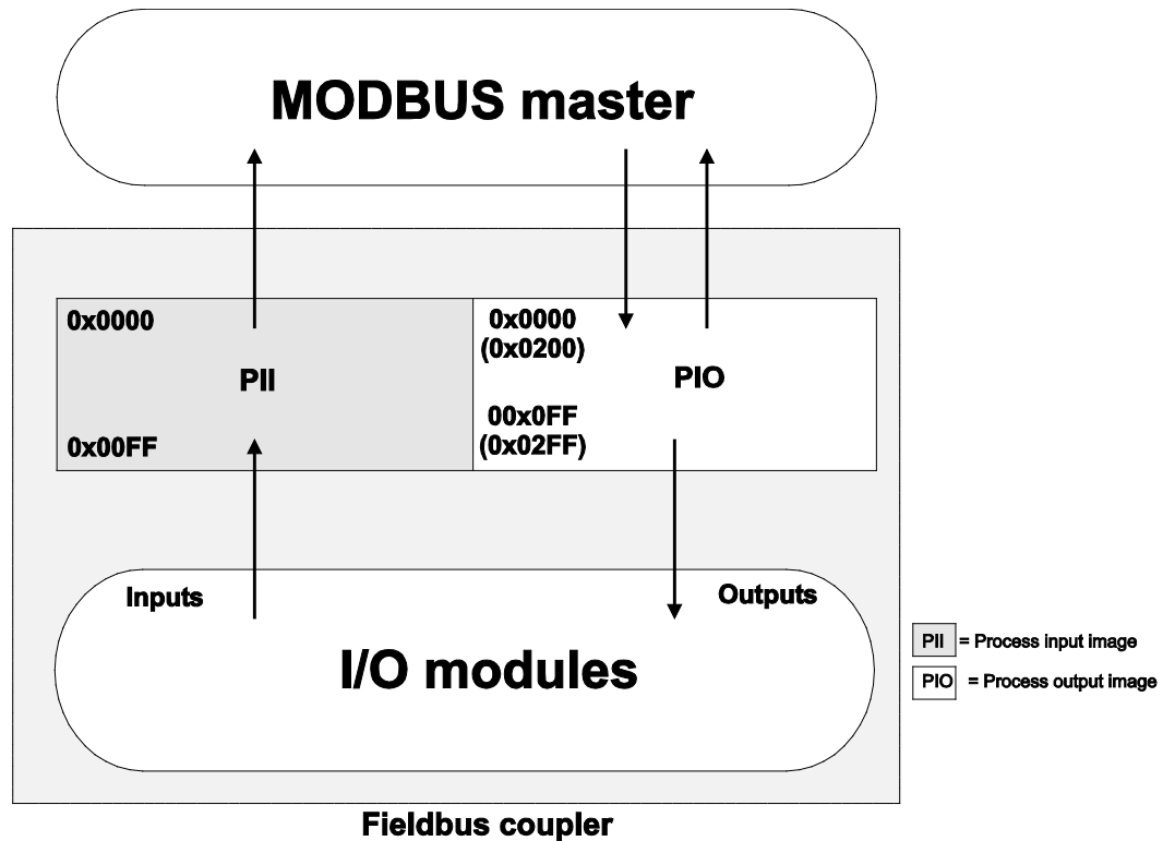
Figure 42: Data Exchange Between the MODBUS Master and the I/O Modules
