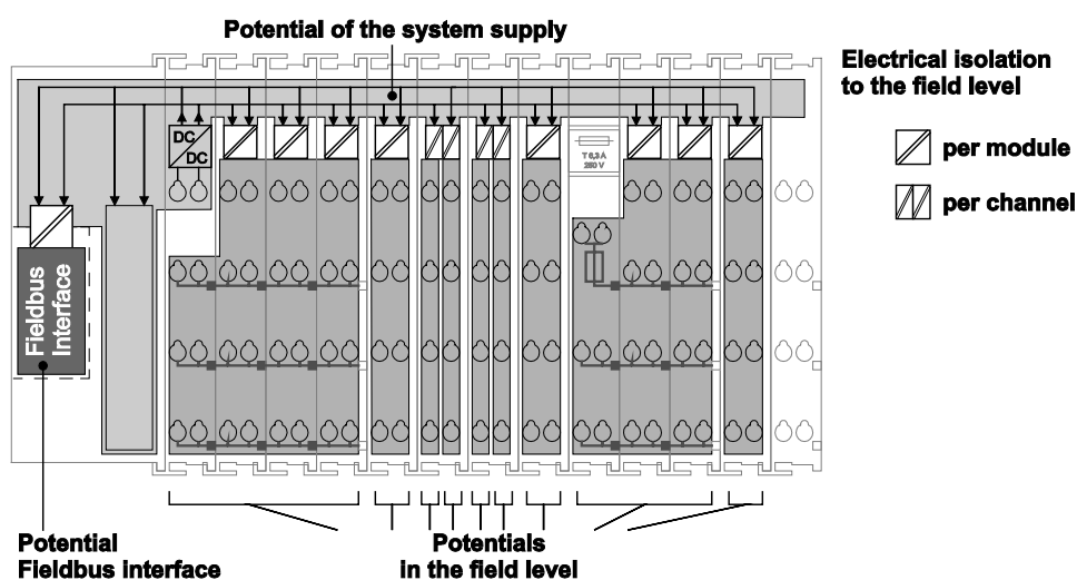
Figure 4: Isolation for Fieldbus Couplers/Controllers (Example)
