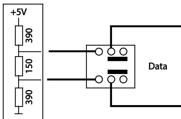
Figure 29: Internal Terminating Resistors and Interface Switches
