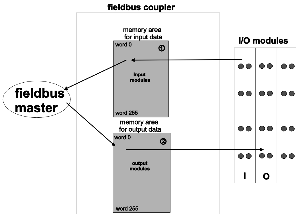
Figure 41: Memory Areas and Data Exchange
