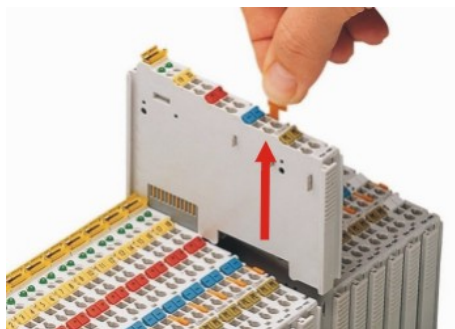
Figure 34: Removing the I/O Module (Example)
