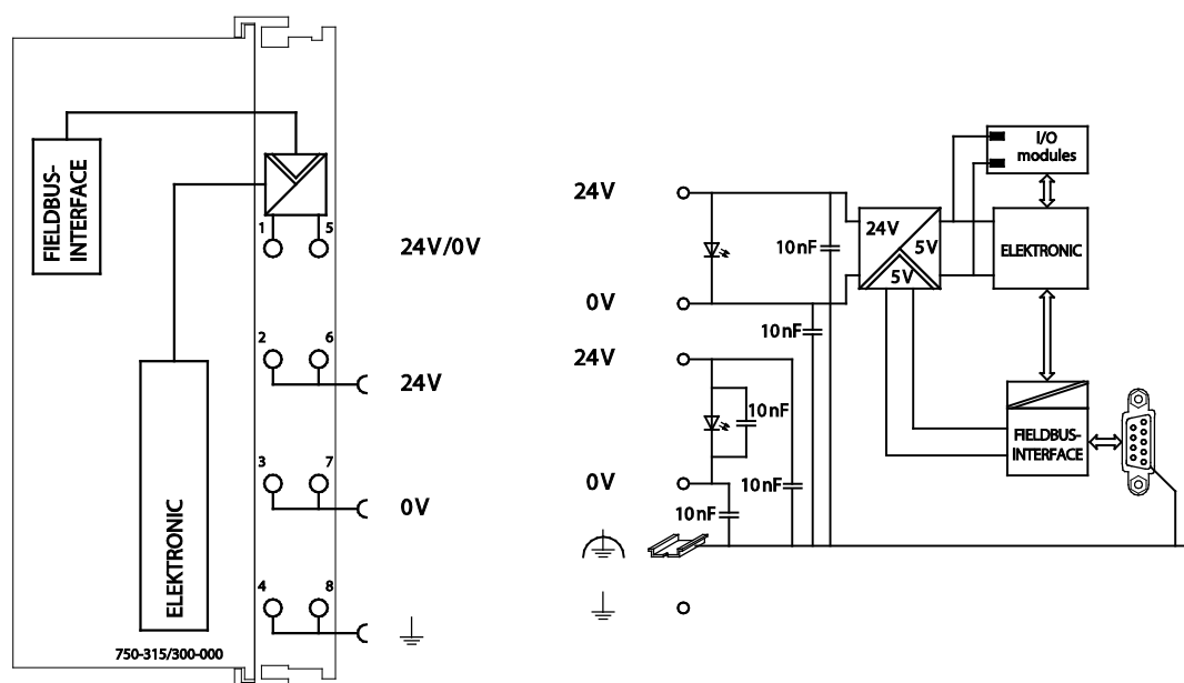
Figure 22: Device Supply
