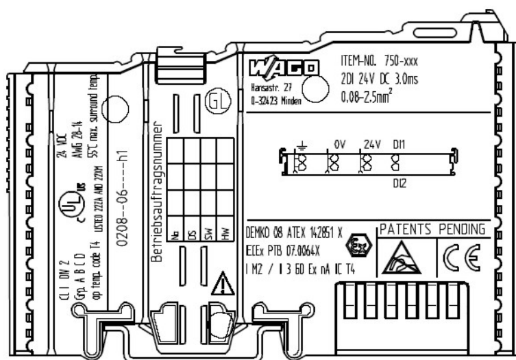
Figure 51: Side Marking Example for I/O Modules According to NEC 500
