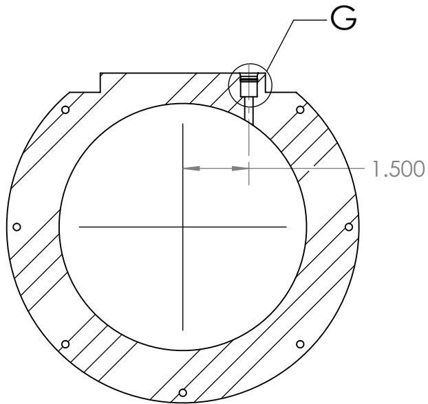
SECTION F-F SCALE 1 : 3
