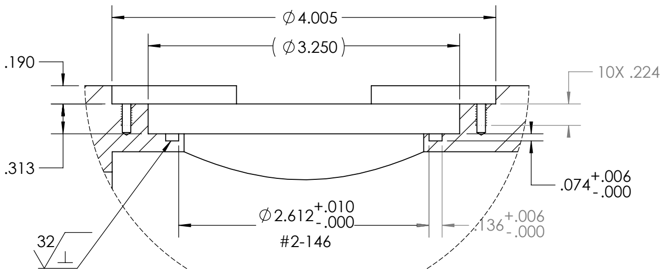
DETAIL D SCALE 1 : 1
