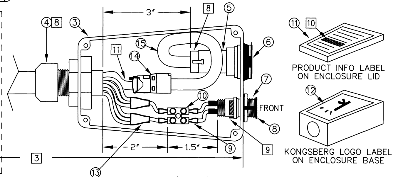
REAR VIEW
