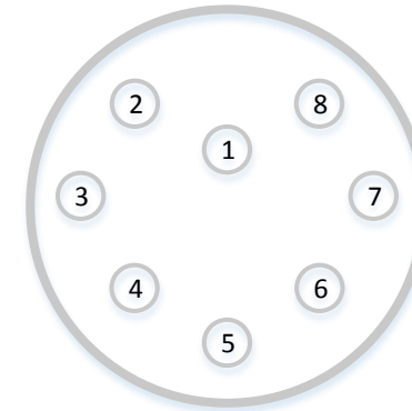
Face view MCBH8F (female)
