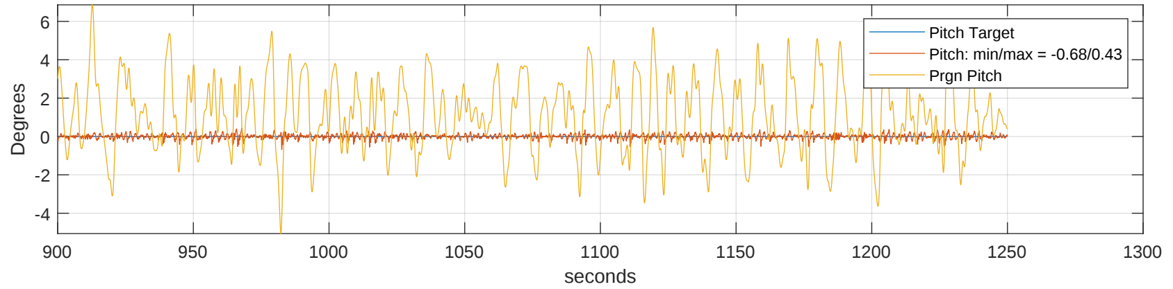
Pitch Motions - Down-Swell
