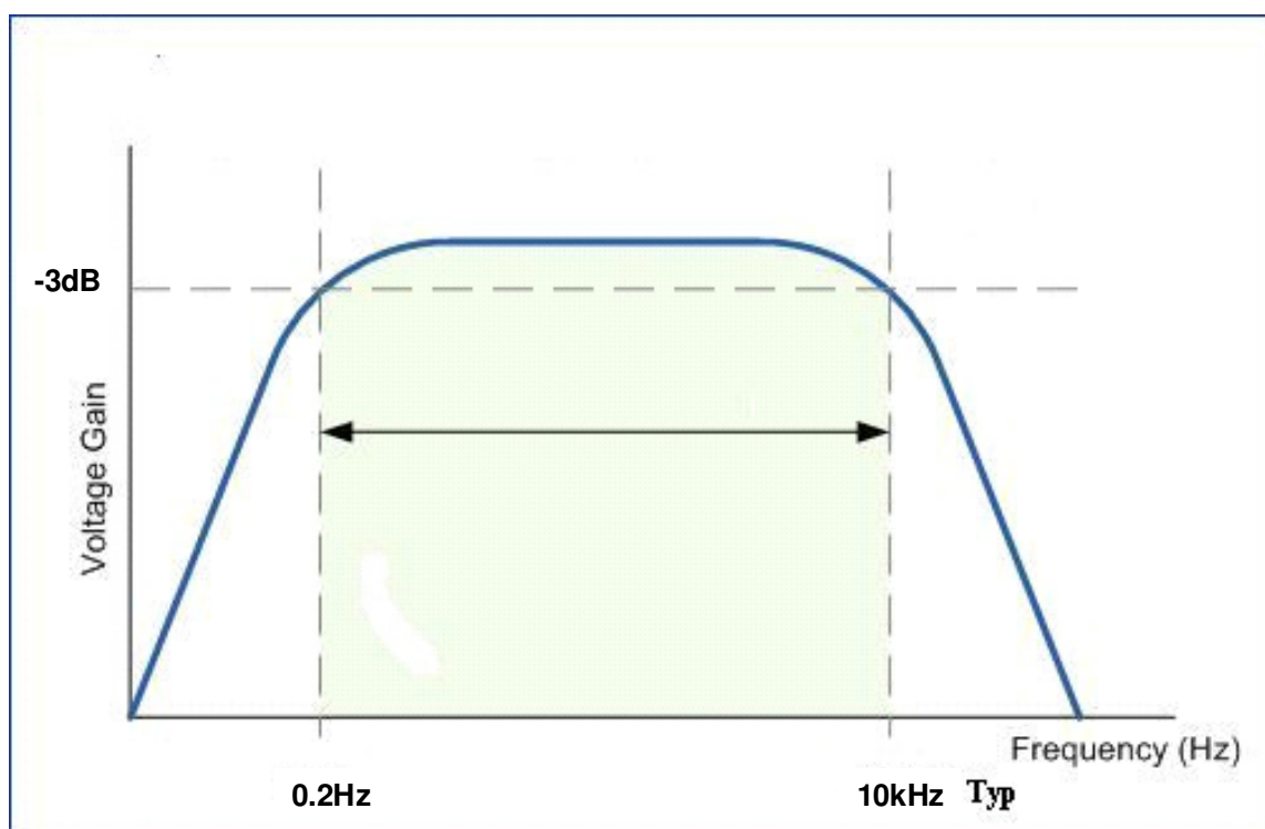
Fig. 3 Typical Bode Plot for PS25451 Sensor with Coupling through 250pF Capacitor
