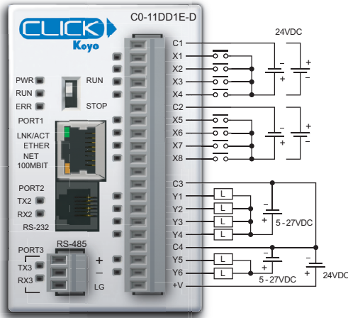
Wiring Diagram
