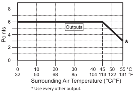
C0-11ARE-D Temperature Derating Chart
