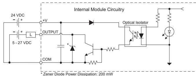
Equivalent Output Circuit
