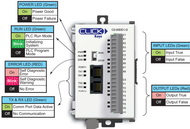
Basic PLC
