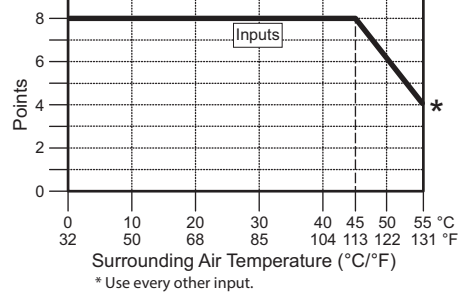
C0-11ARE-D Temperature Derating Chart
