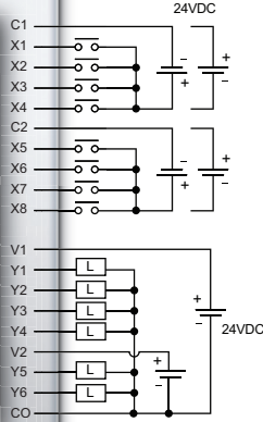
Wiring Diagram
