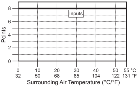
C0-01AR-D Temperature Derating Chart
