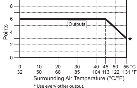
C0-10DD2E-D Temperature Derating Chart
