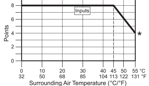
C0-11DD1E-D Temperature Derating Chart
