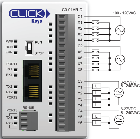
Wiring Diagram
