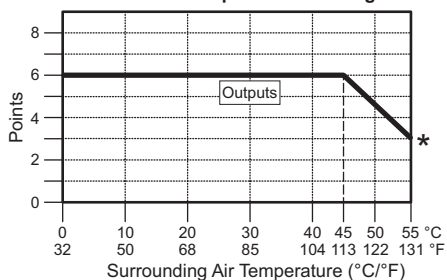
C0-10DRE-D Temperature Derating Chart
