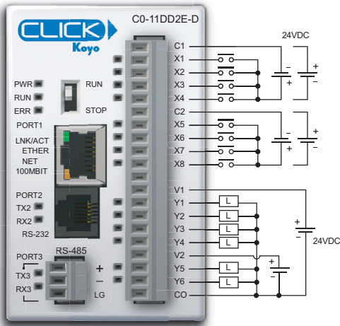
Wiring Diagram
