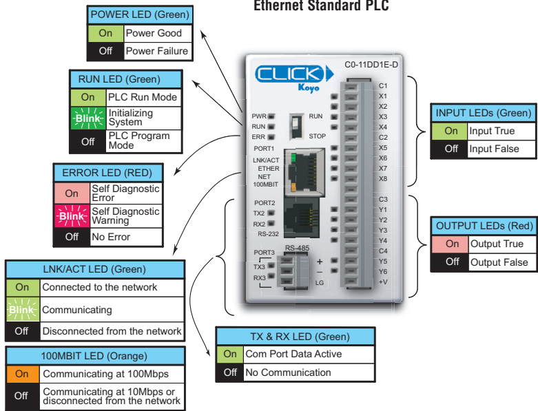
Ethernet Standard PLC
