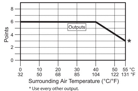
C0-00AR-D Temperature Derating Chart
