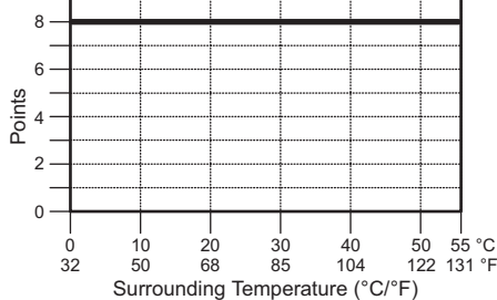
Input Module Temperature Derating Chart
