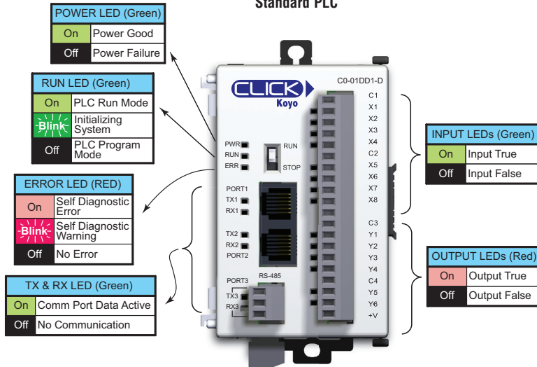
Standard PLC
