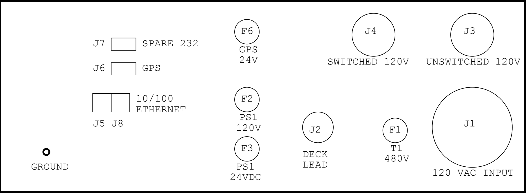
REAR PANEL LAYOUT
