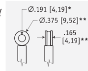
eyelet detail
