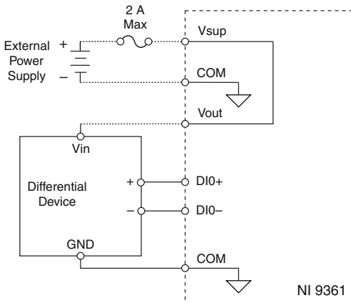
Figure 5. Connecting a Differential Device
