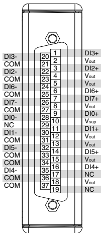
Figure 1. NI 9361 Pinout
