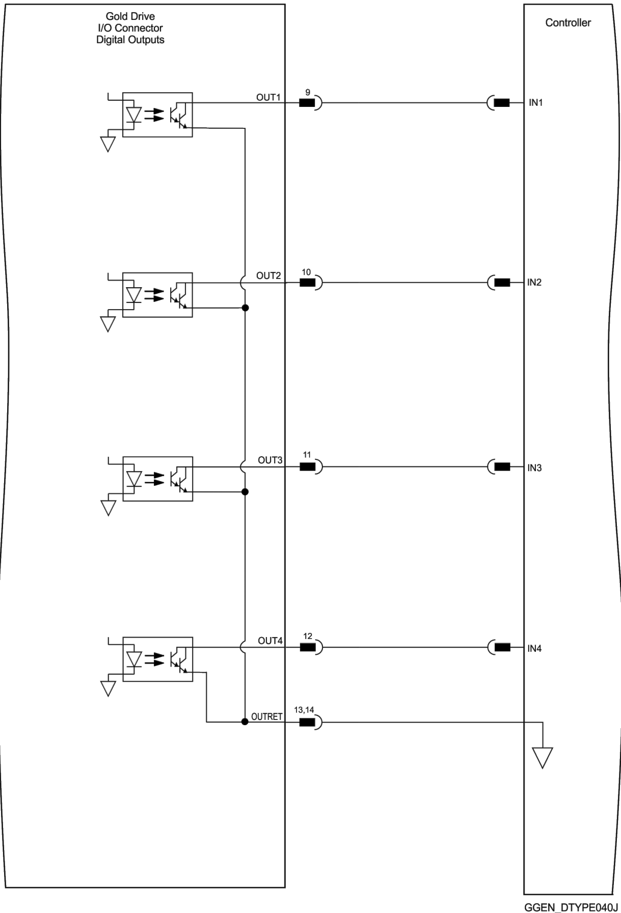
Figure 40: Digital Output Connection Diagram Example – Sink PLC Option
