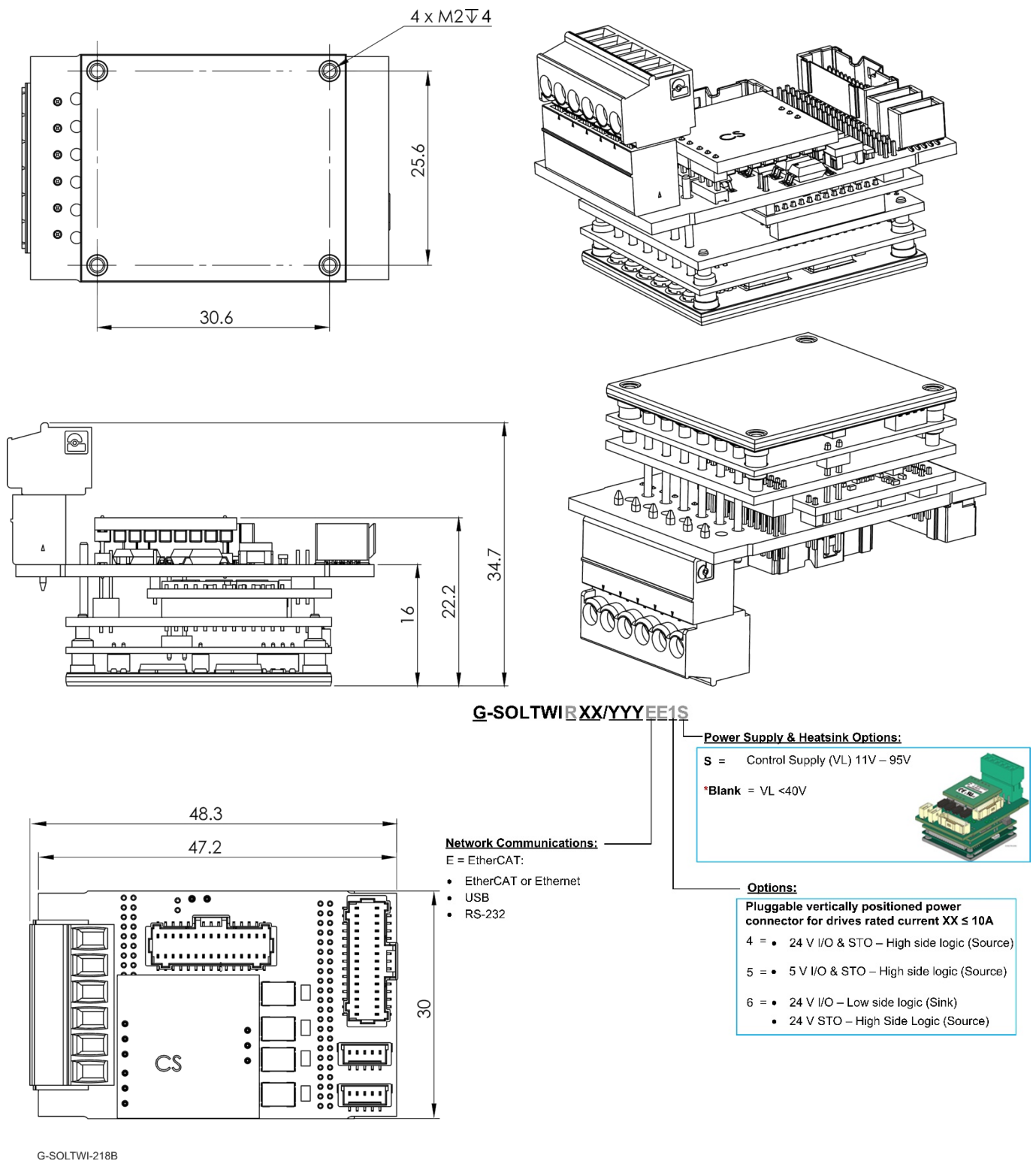
Figure 55: G-Solo Twitter –EtherCAT version with vertical power connector
