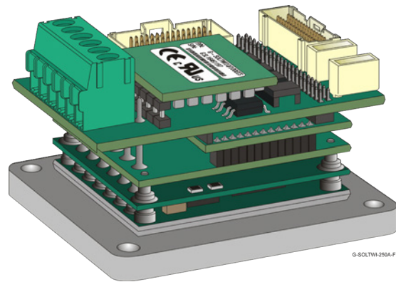
Flat Heat Sink (P/N G-TWIHSFLAT01)
