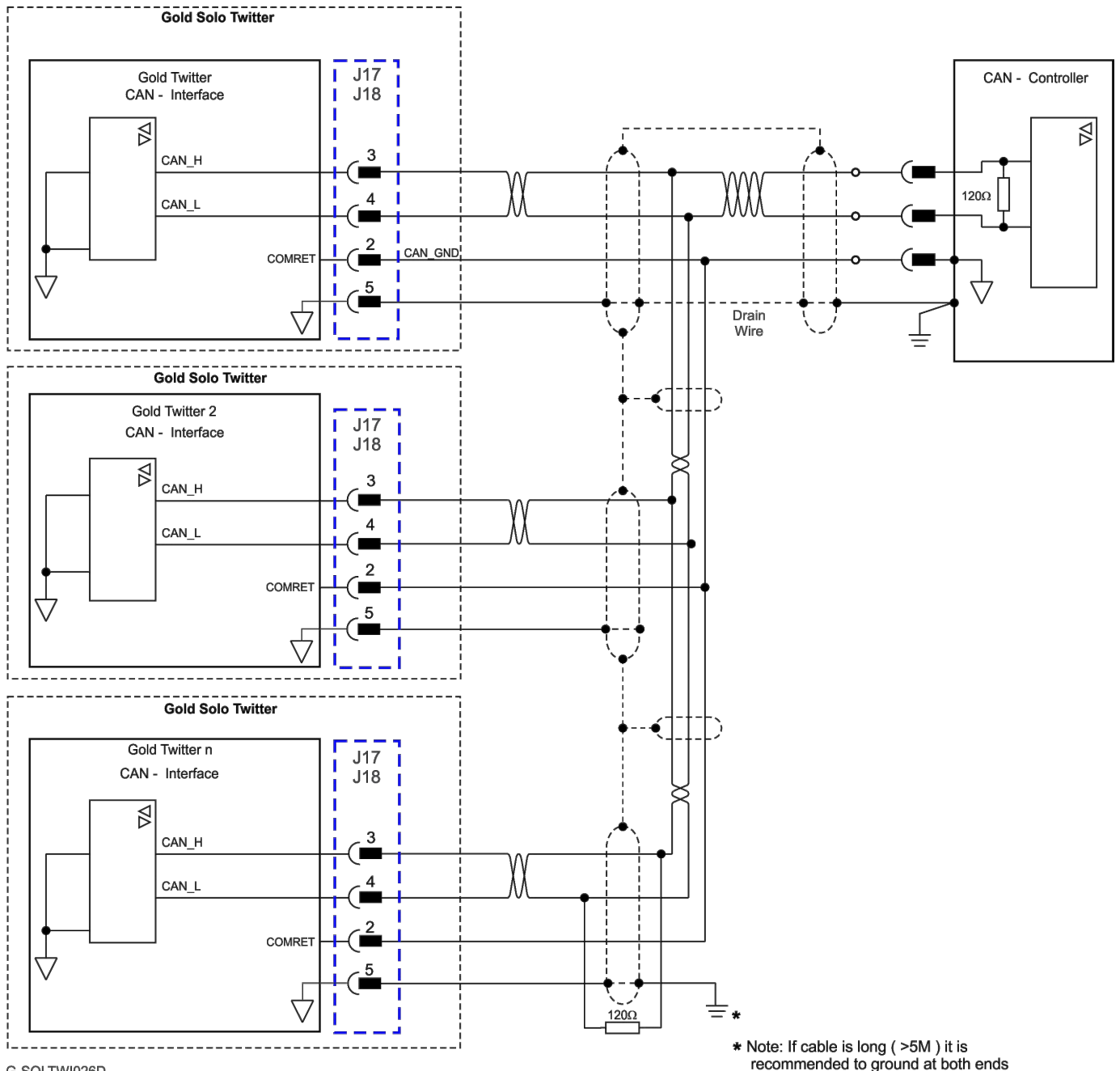
Figure 52: CAN Network Diagram – Drop Off Topology
