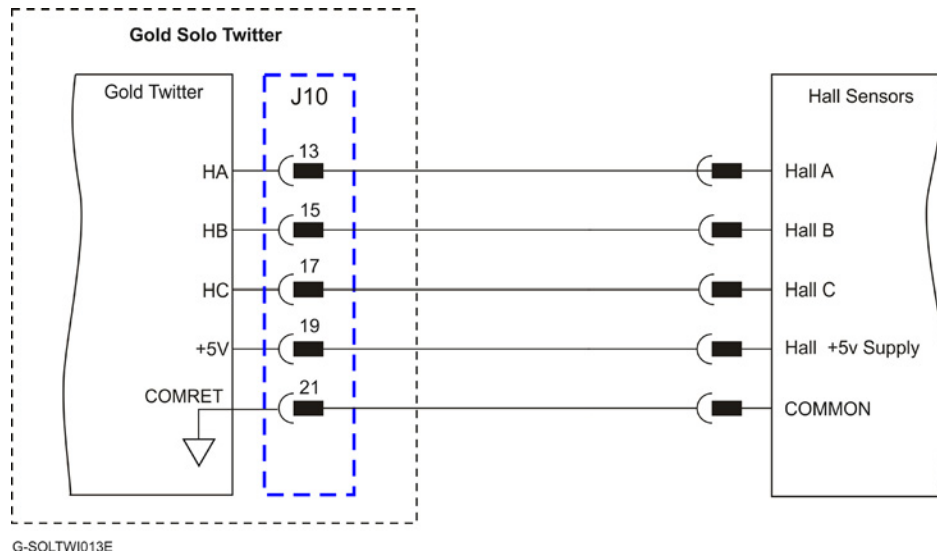
Figure 25: Hall Sensors Connection Diagram
