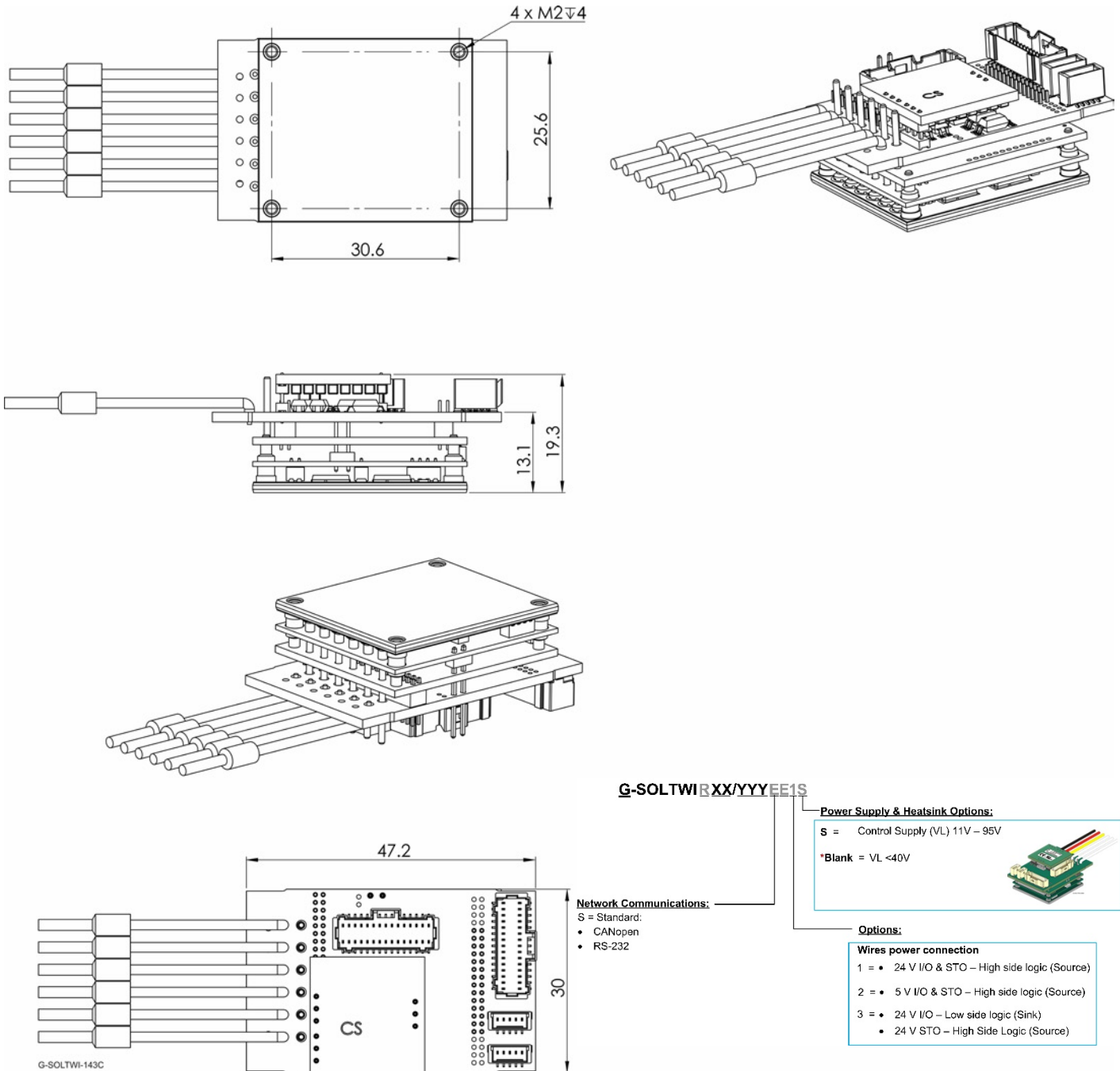
Figure 59: G-Solo Twitter –CAN version with wires to power supply and motor
