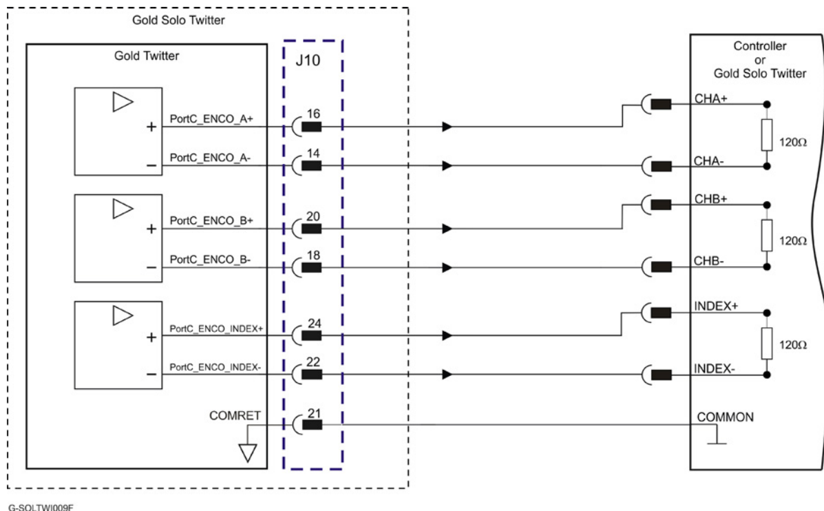
Figure 29: Emulated Encoder Differential Output – Recommended Connection Diagram
