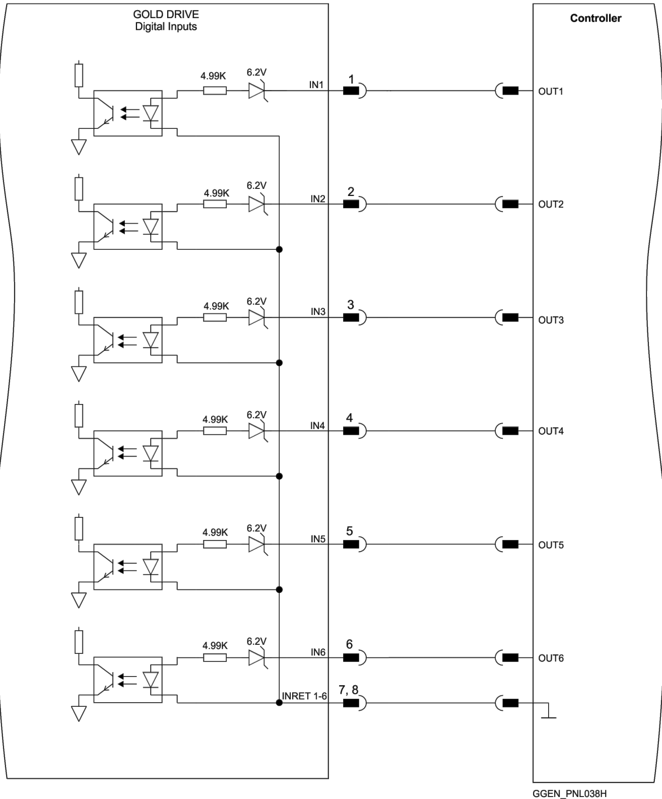
Figure 32: Digital Input Connection Diagram Example – Source PLC Option
