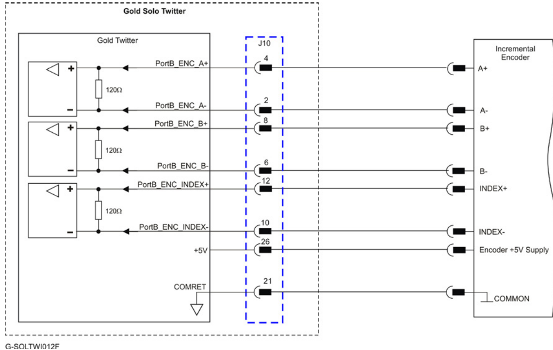
Figure 26: Port B Incremental Encoder Input – Recommended Connection Diagram
