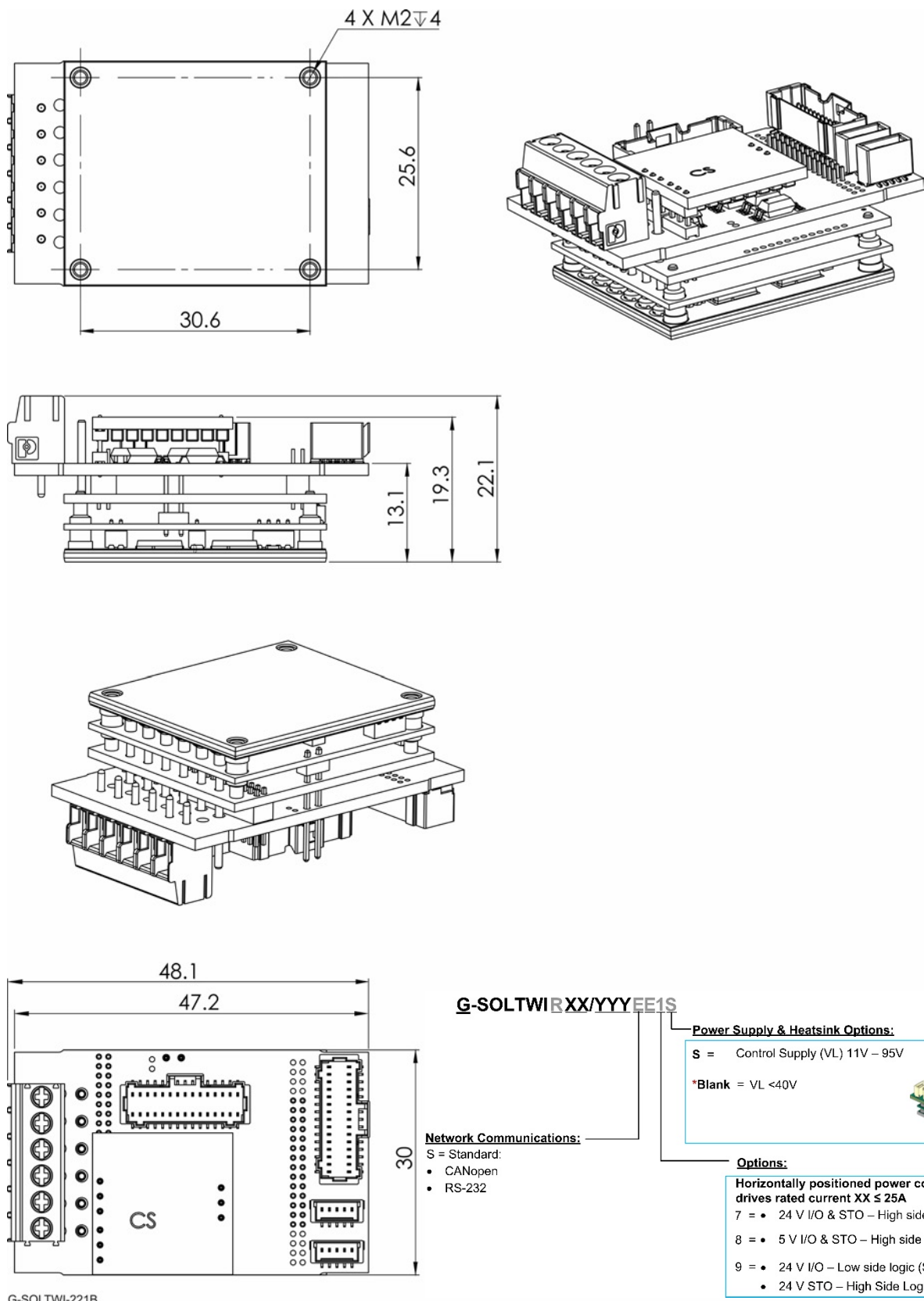
Figure 60: G-Solo Twitter –CAN version with horizontal power connector
