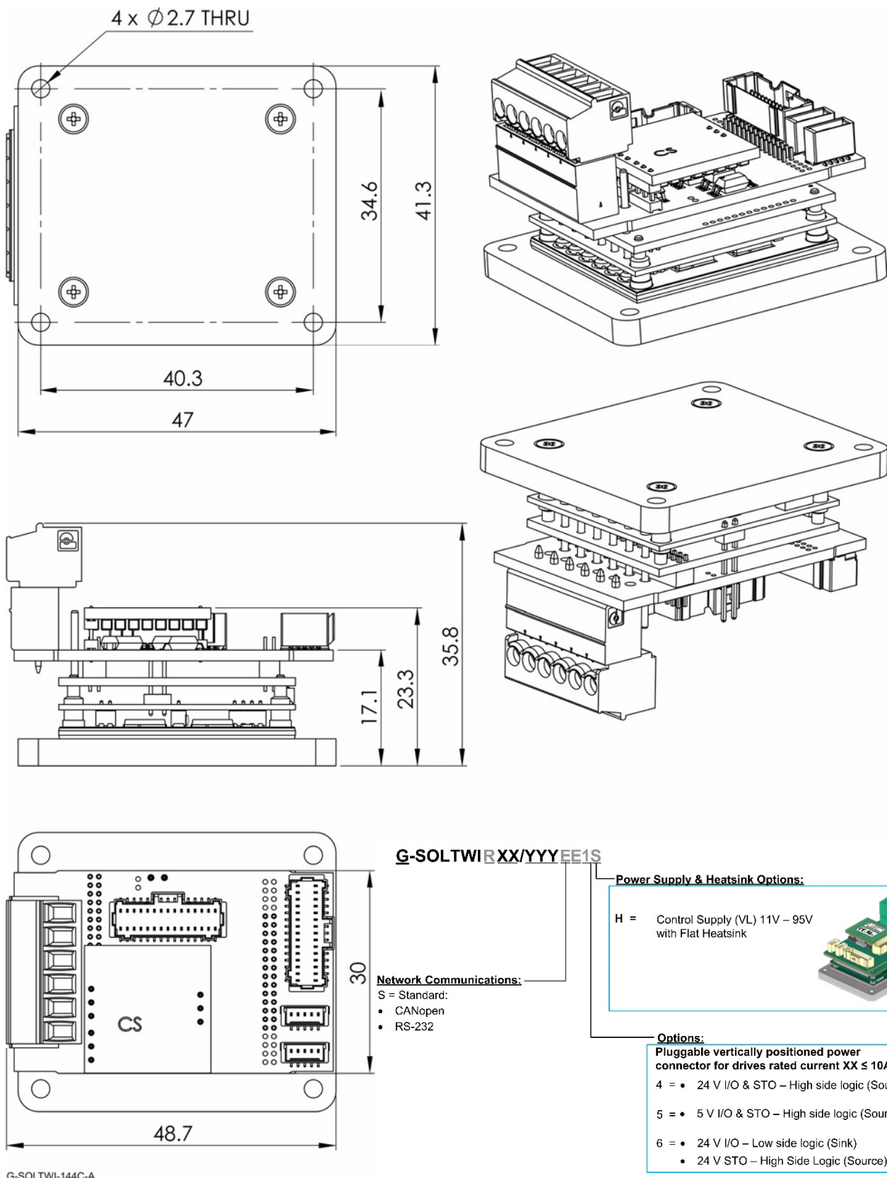
Figure 64: G-Solo Twitter –CAN version with vertical power connector
