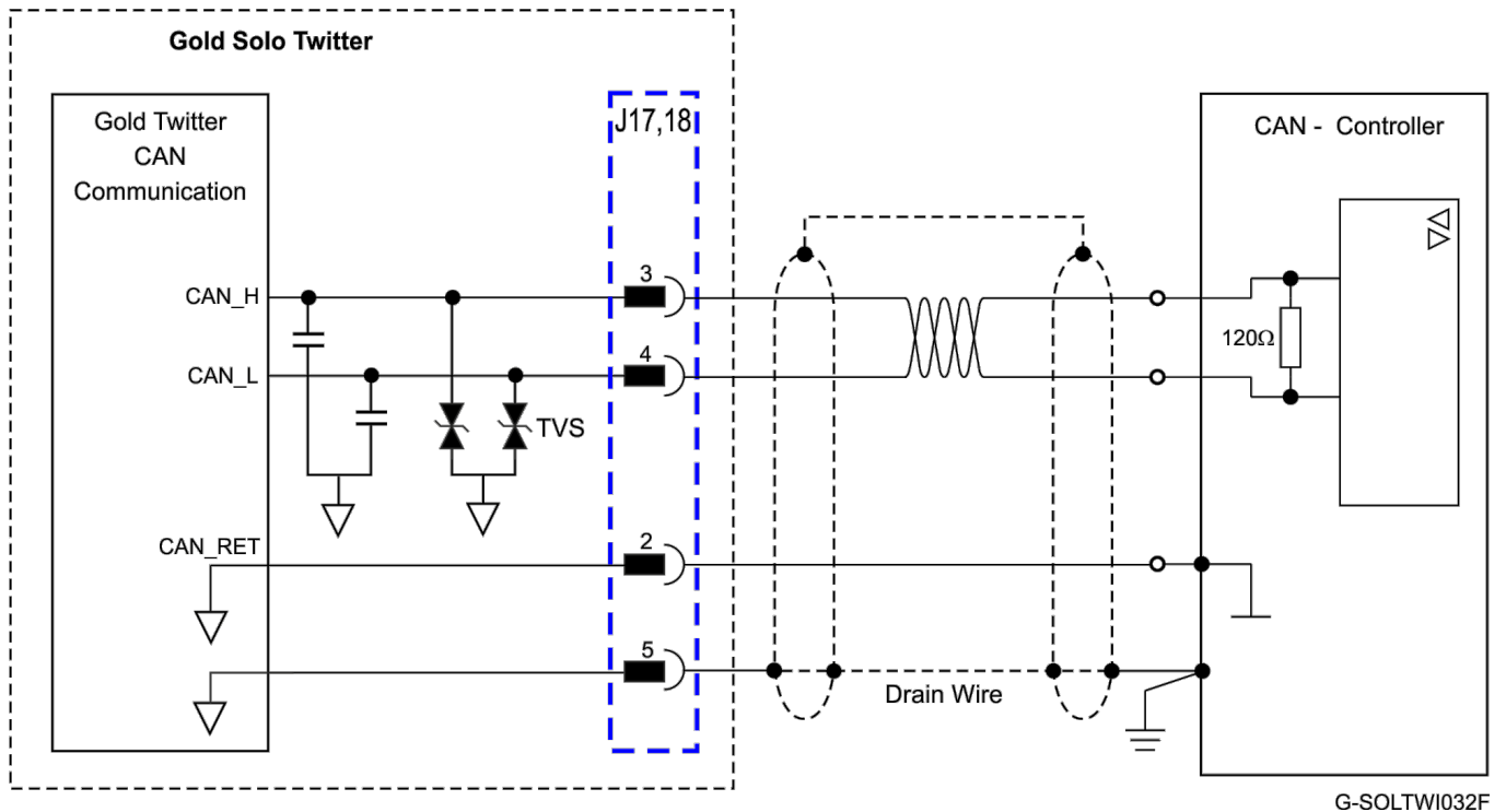
Figure 51: CAN Interface
