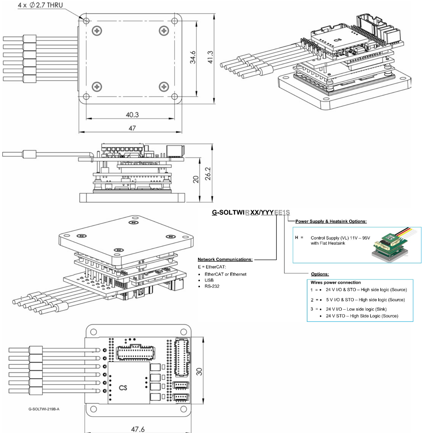
Figure 56: G-Solo Twitter –EtherCAT version with wires to power supply and motor
