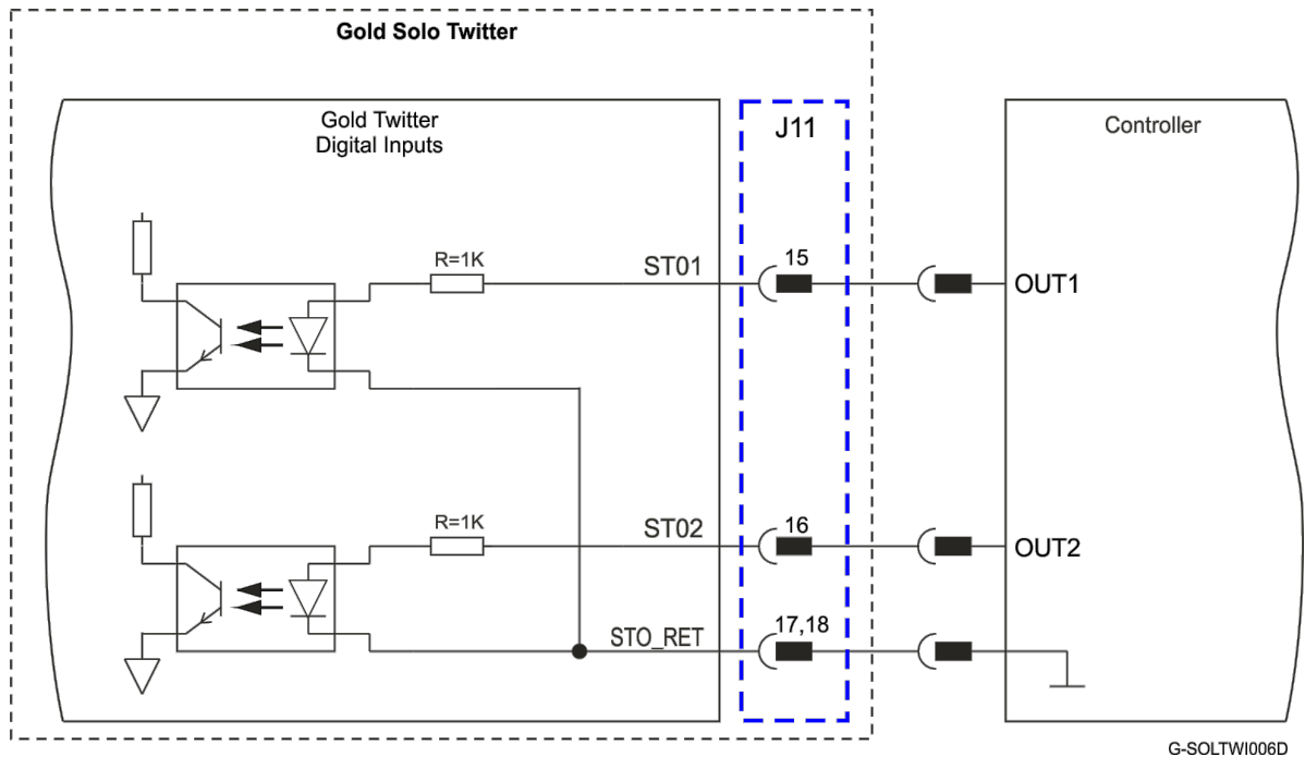
Figure 43: STO Input Connection – 5V Logic
