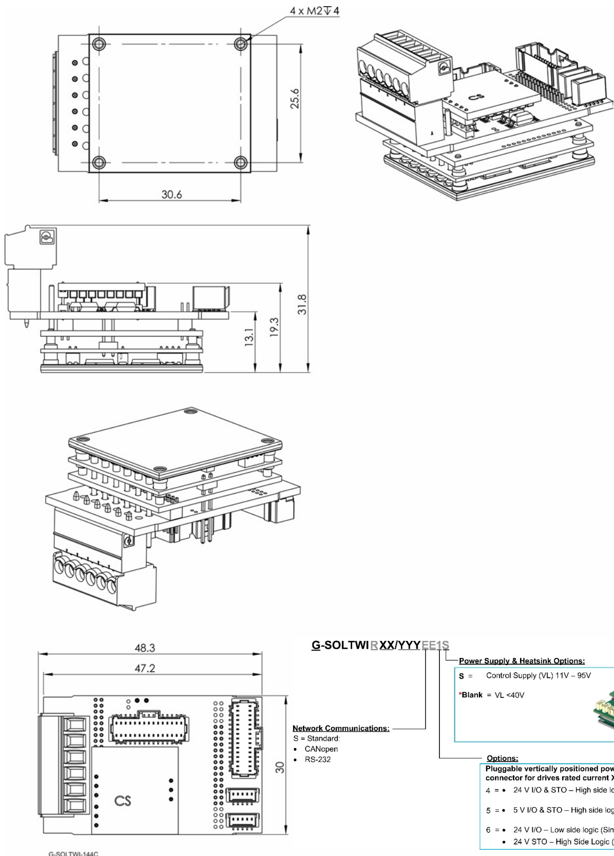
Figure 61: G-Solo Twitter –CAN version with vertical power connector
