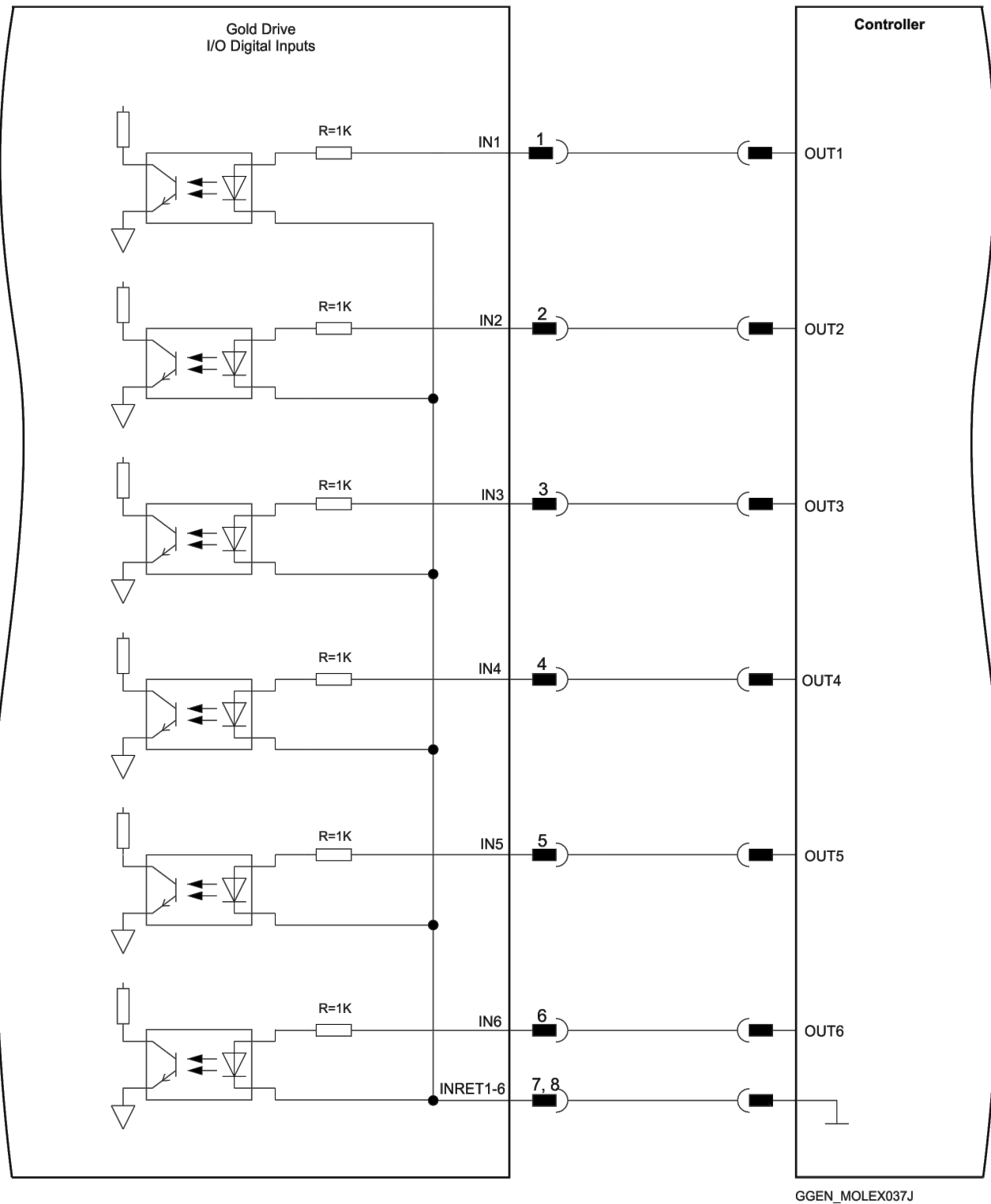
Figure 36: Digital Input Source 5V Logic Mode Connection Diagram
