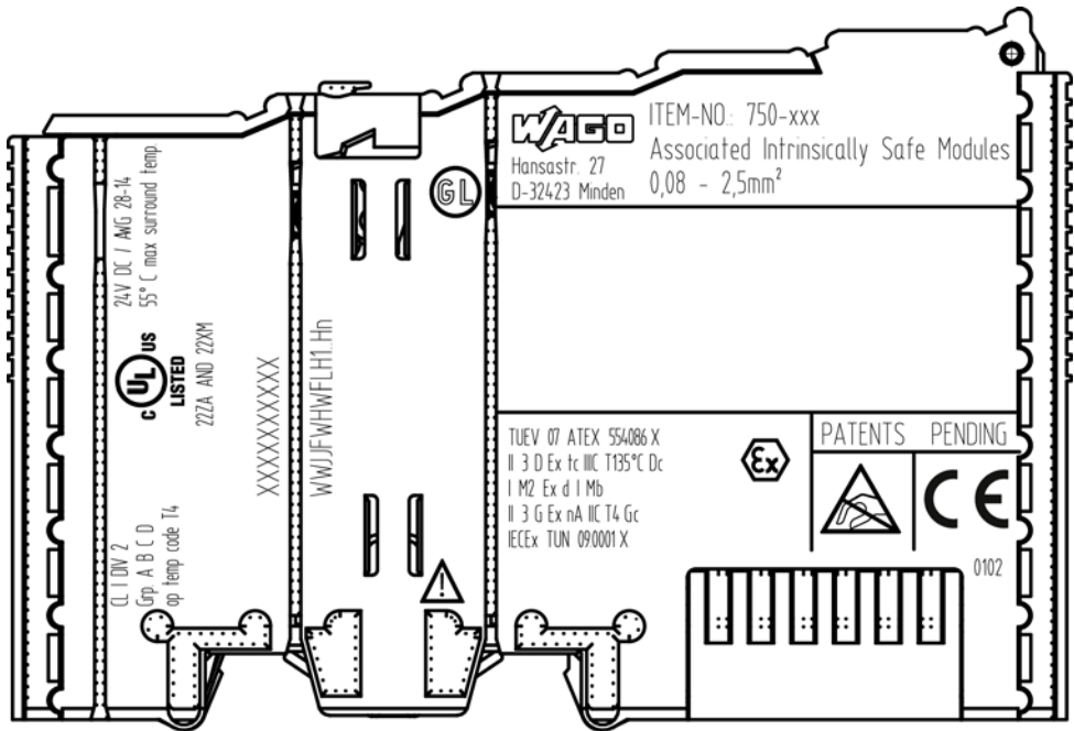
Figure 47: Marking Example According to NEC
