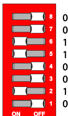
Figure 38: Address Selection Switch, for Example the Value Setting "50" ( 2^1 + 2^4 + 2^5 )
