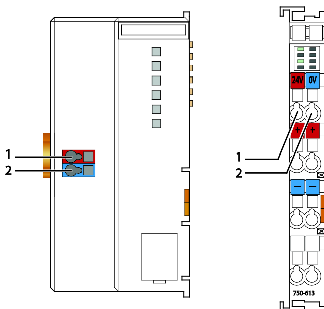
Figure 5: System Supply
