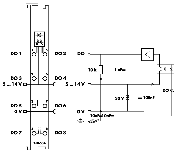
Figure 6: Schematic Diagram
