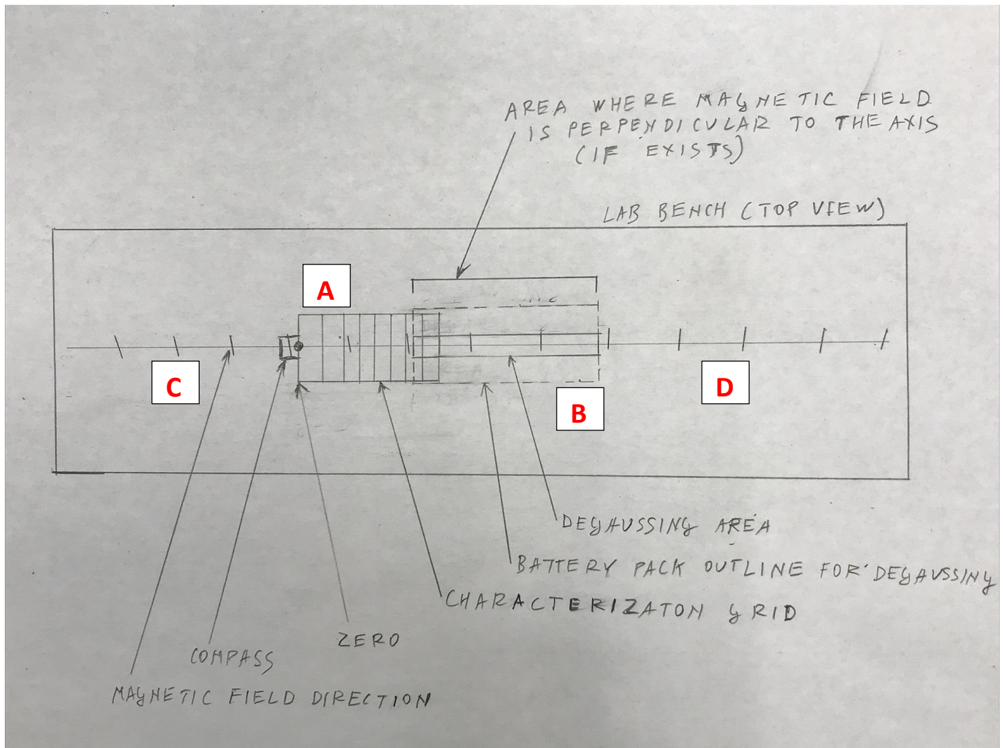
Fig 1. Schematic diagram of a typical setup to characterize and degauss a battery pack (or other components), Top View A: Characterization grid. B: Degaussing area. C: Lines, visualizing Earth's magnetic field direction along the axis of the table D: "Magnetic Infinity" area
