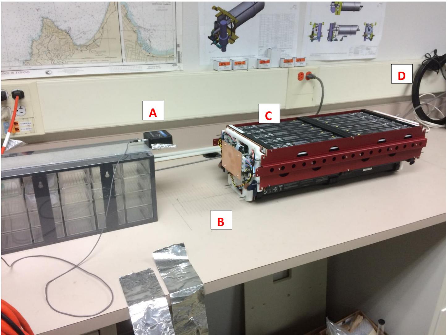
Fig 4. Characterization setup, typical [Example 1]
