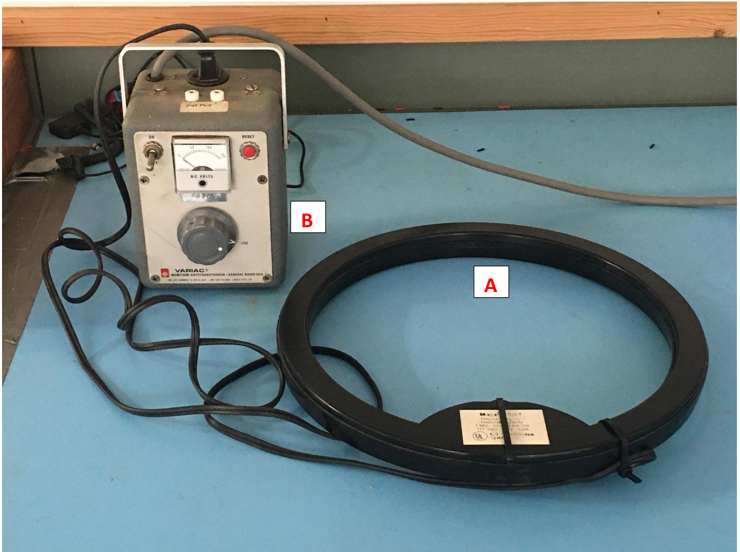
Fig 9. Degaussing coil example
