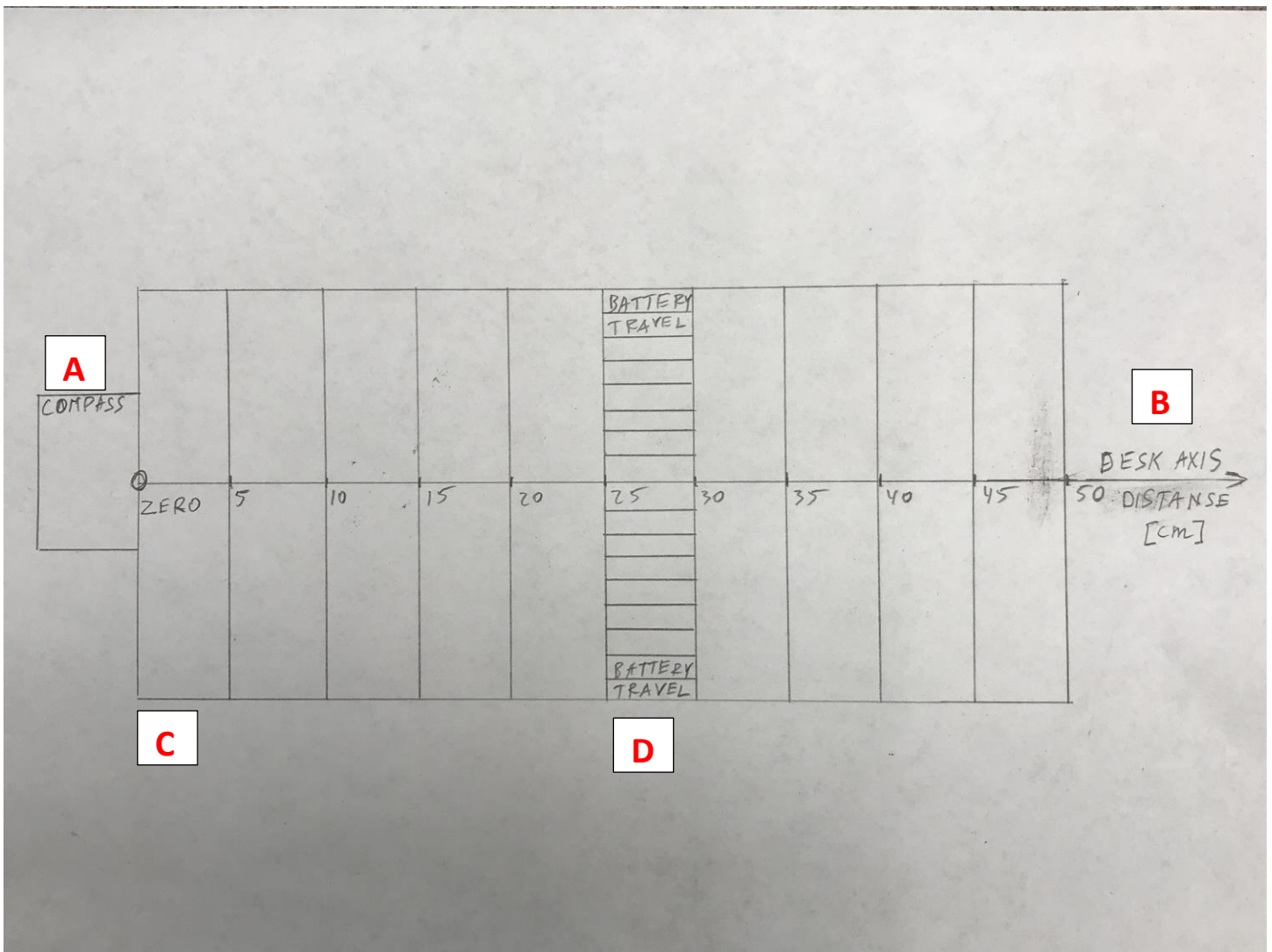
Fig 2. Schematic diagram of Characterization Grid, inscribed on the lab bench (Top View)
