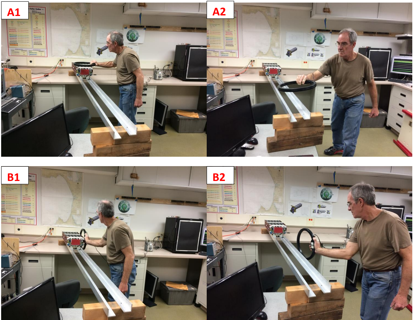
Fig 16. Example of degaussing sequence A1-A2: degaussing Top surface B1-B2: degaussing Port surface
