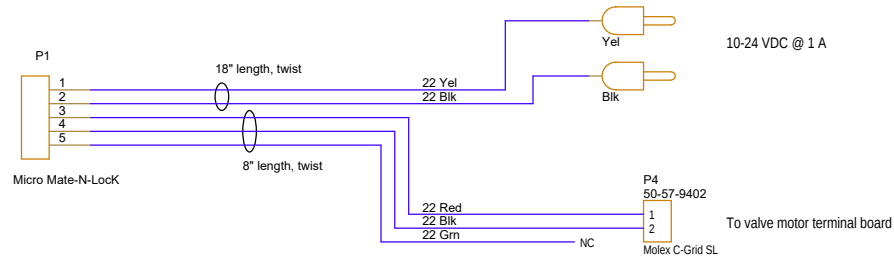
Motor and Power Connector J1
