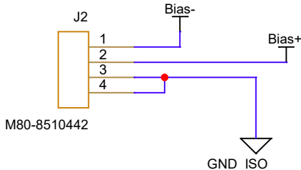
DuraFET isolated Bias power
