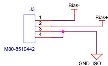
DuraFET isolated Bias power
