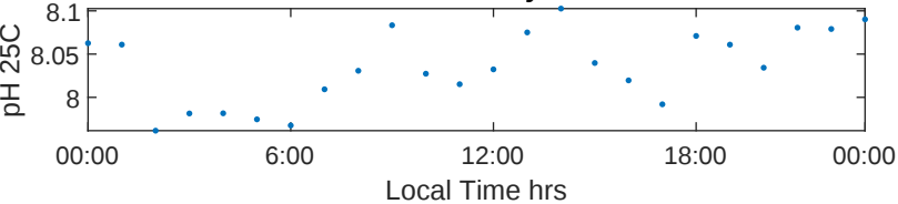
mean diel cycle
