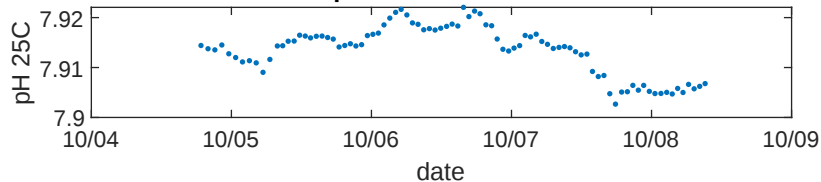
pH full time series
