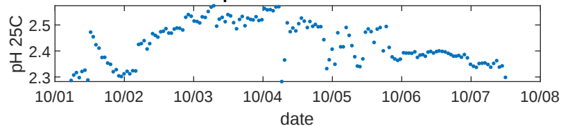
pH full time series
