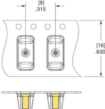
0305-2-57 Tape & Reel Details
