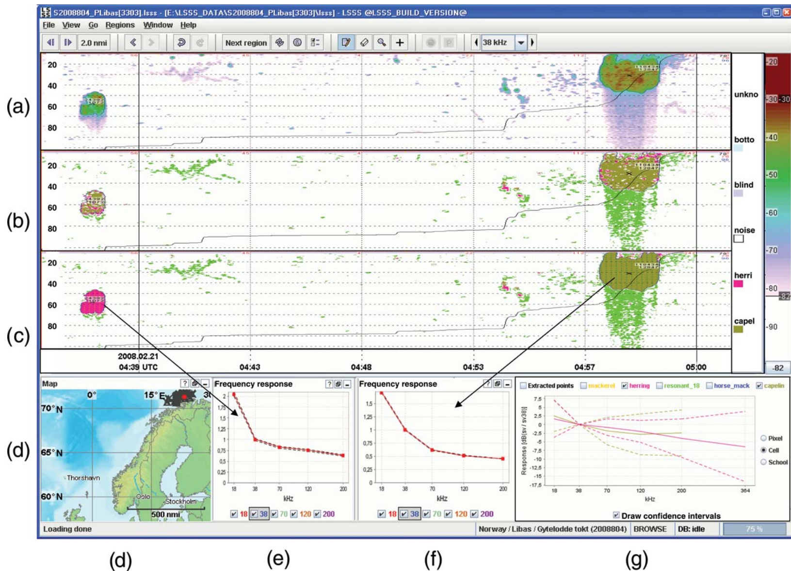
Figure 3. Echograms (a–c) and auxiliary information (d–g) used during data interpretation. Colour scales indicating backscattering strength and acoustic categories appear to the right of the echograms. (a) Smoothed and noise-corrected echograms at 38 kHz; (b) pixel- and (c) school-based acoustic identification combined with geographical restrictions; (d) map of the surveyed area; (e and f) relative frequency response of the arrowed schools identified as herring and capelin, respectively; (g) the training database illustrating the relative frequency responses with confidence intervals in school cells for herring and capelin.
