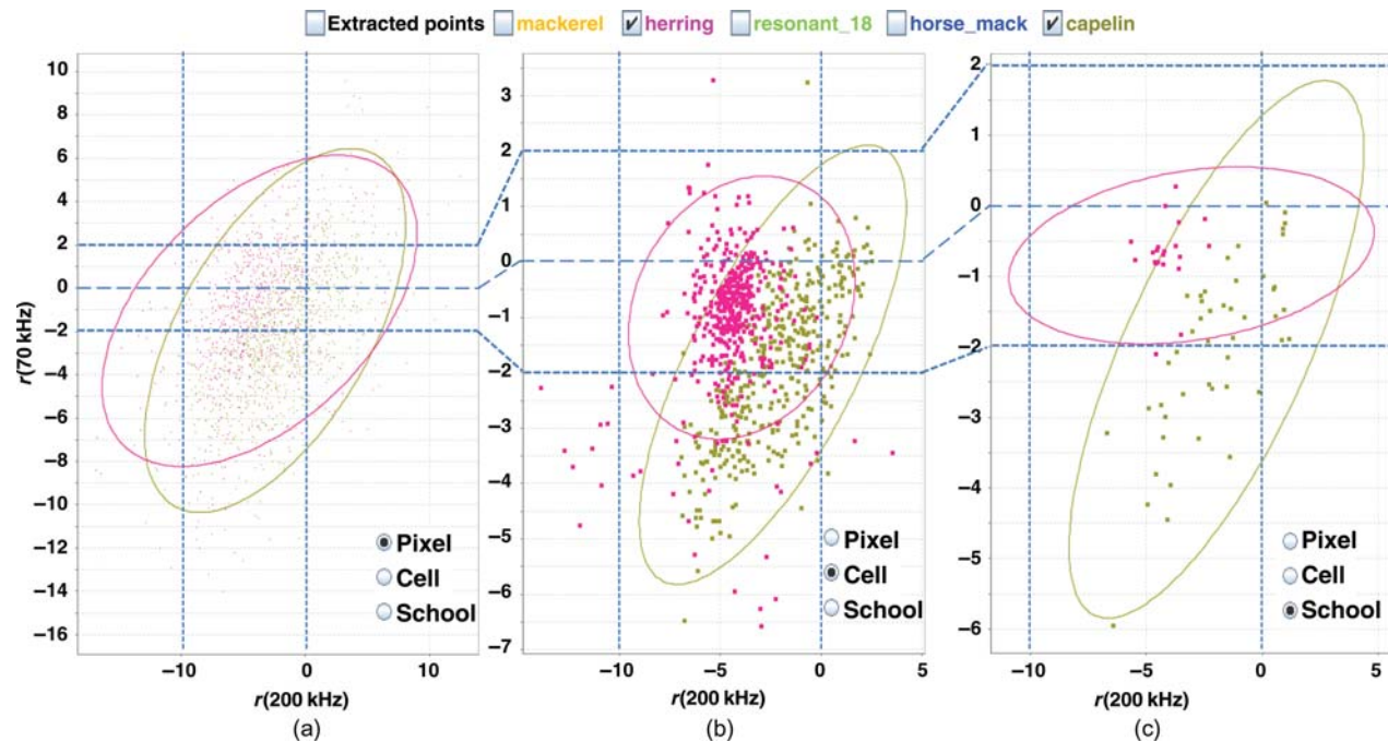
Figure 1. The relative frequency response r(70 \text{ kHz}) against r(200 \text{ kHz}) from the training dataset for the categories “herring” and “capelin” at different scales: (a) elementary volumes, (b) cell, and (c) entire schools. The data are taken from the complete library of acoustic data used for the identification of acoustic categories (= “species”) and have been verified by biological samples.
