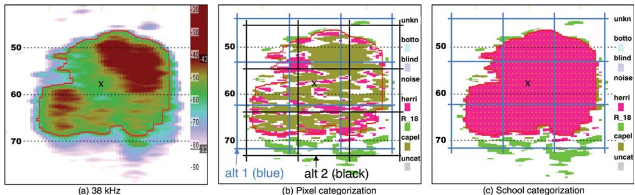
Figure 4. Comparison of categorization levels. (a) Echogram at 38 kHz, smoothed s_r ; (b) the pixel-based categorization displays two alternative placements of the cells; (c) the school-based categorization has a unique result.
