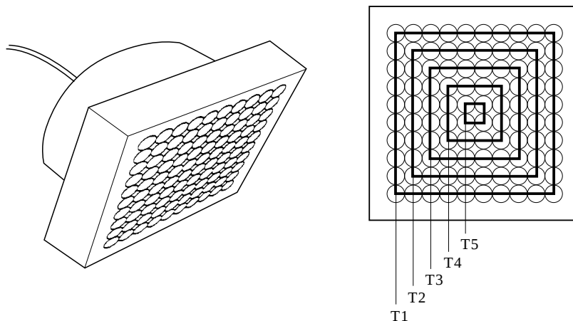
Figure 1. Transducer element arrangements.
