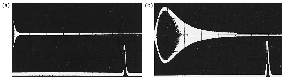
Figure 2. Real-time pulse compression, oscillogram examples. Top traces = transmitted signal, bottom traces = processing output, horizontal scale: 2 ms/division. (a) Short low-frequency signal ( B=20\text{--}40\text{ kHz} , T=1\text{ ms} ), (b) long high-frequency signal ( B=60\text{--}80\text{ kHz} , T=10\text{ ms} ).
