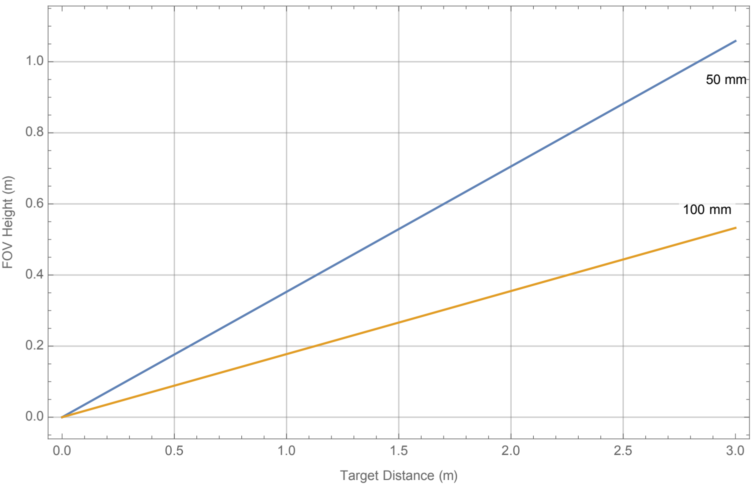
Field-of-View Height vs. Target Distance For Coral Obs Macro Camera
