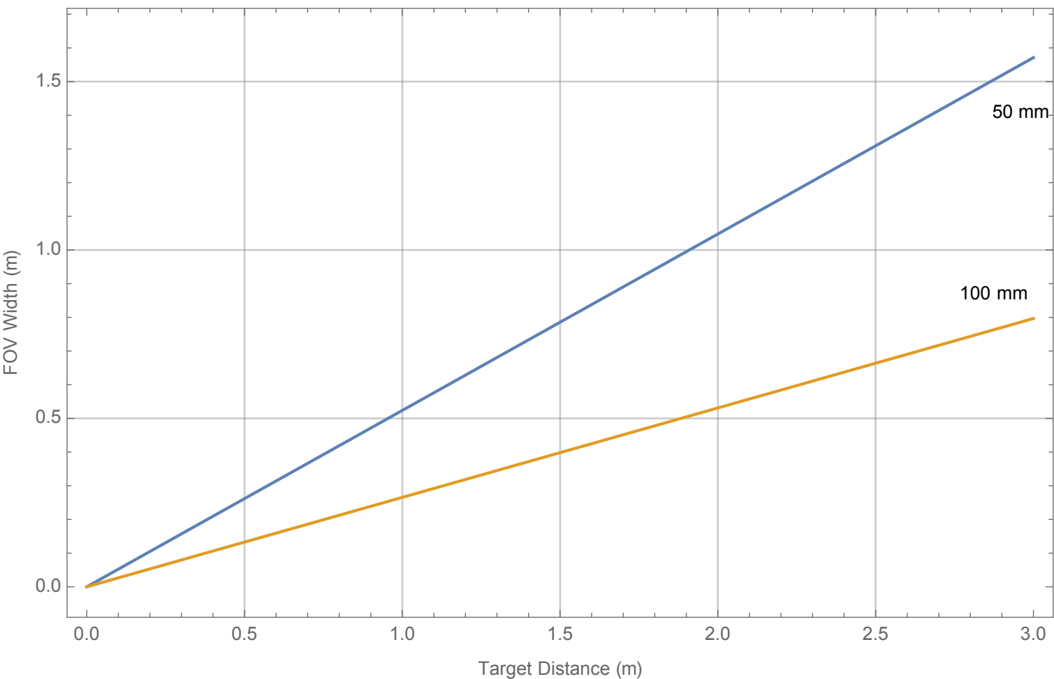
Field-of-View Width vs. Target Distance For Coral Obs Macro Camera
