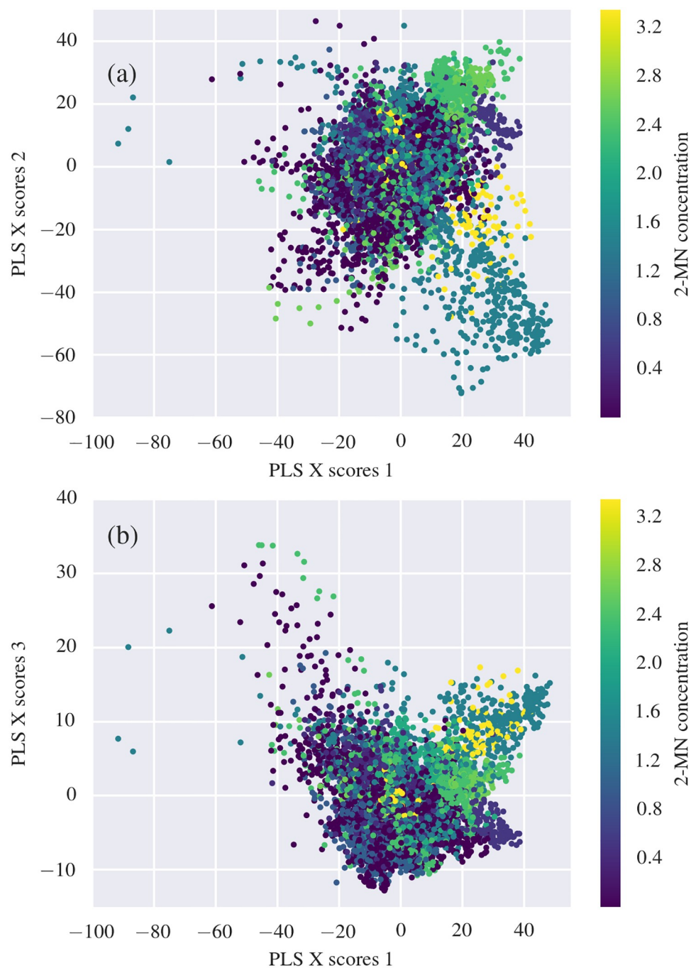
Fig 8. PLS scores for white corals. (a) shows scores for X latent variable 1 vs latent variable 2, (b) shows scores for X latent variable 1 vs latent variable 3. One dot corresponds to one spectrum (i.e. one hyperspectral image pixel) taken from a coral.
