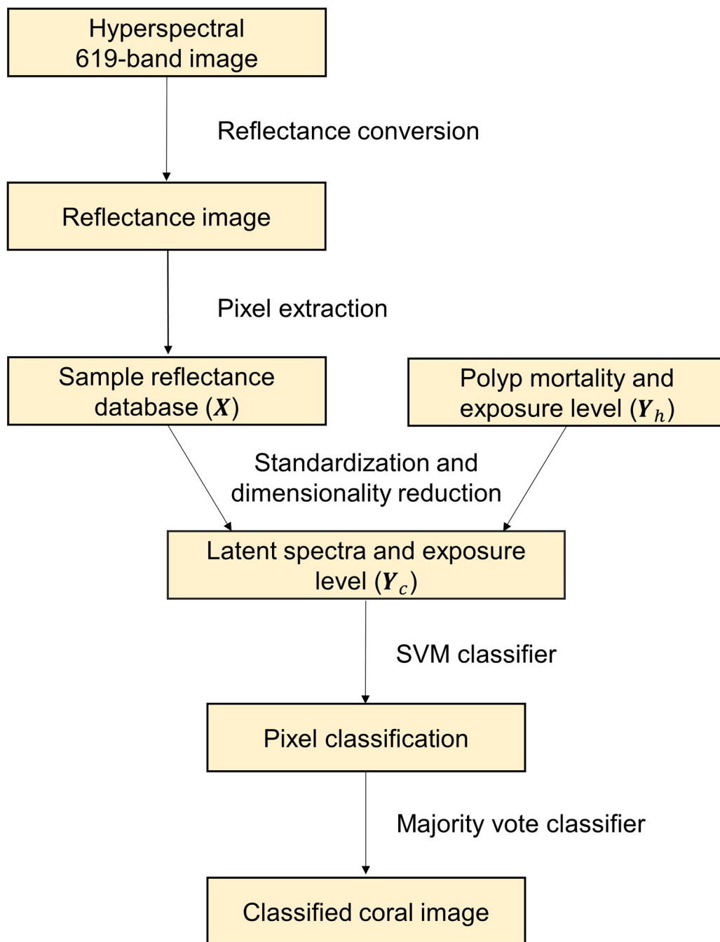
Fig 4. Data analysis flowchart. The flowchart shows the full data analysis pipeline including all steps of the classification model.
