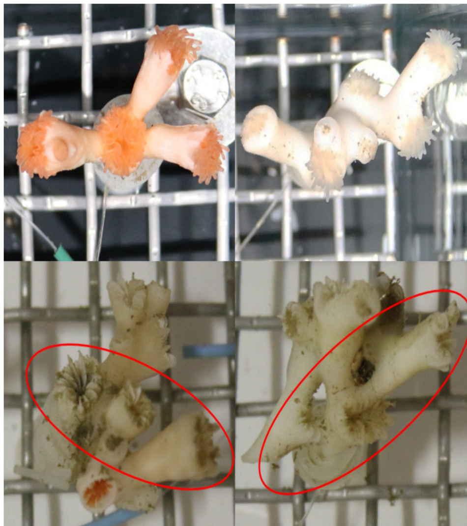
Fig 2. Example images of living and dead corals. Example images of alive and dead polyps. Upper row—pictures from time 0 h: orange and white coral samples with healthy polyps. Lower row—pictures from time 1440 h: orange and white coral samples with dead polyps (red ellipse indicates dead polyps). The coral sample in the lower left picture was orange prior to exposure, but exposure to 2-methylnaphthalene lead to loss of pigmented tissue and has rendered it predominantly white. The lower right picture exhibits a white coral sample with dead polyps.
