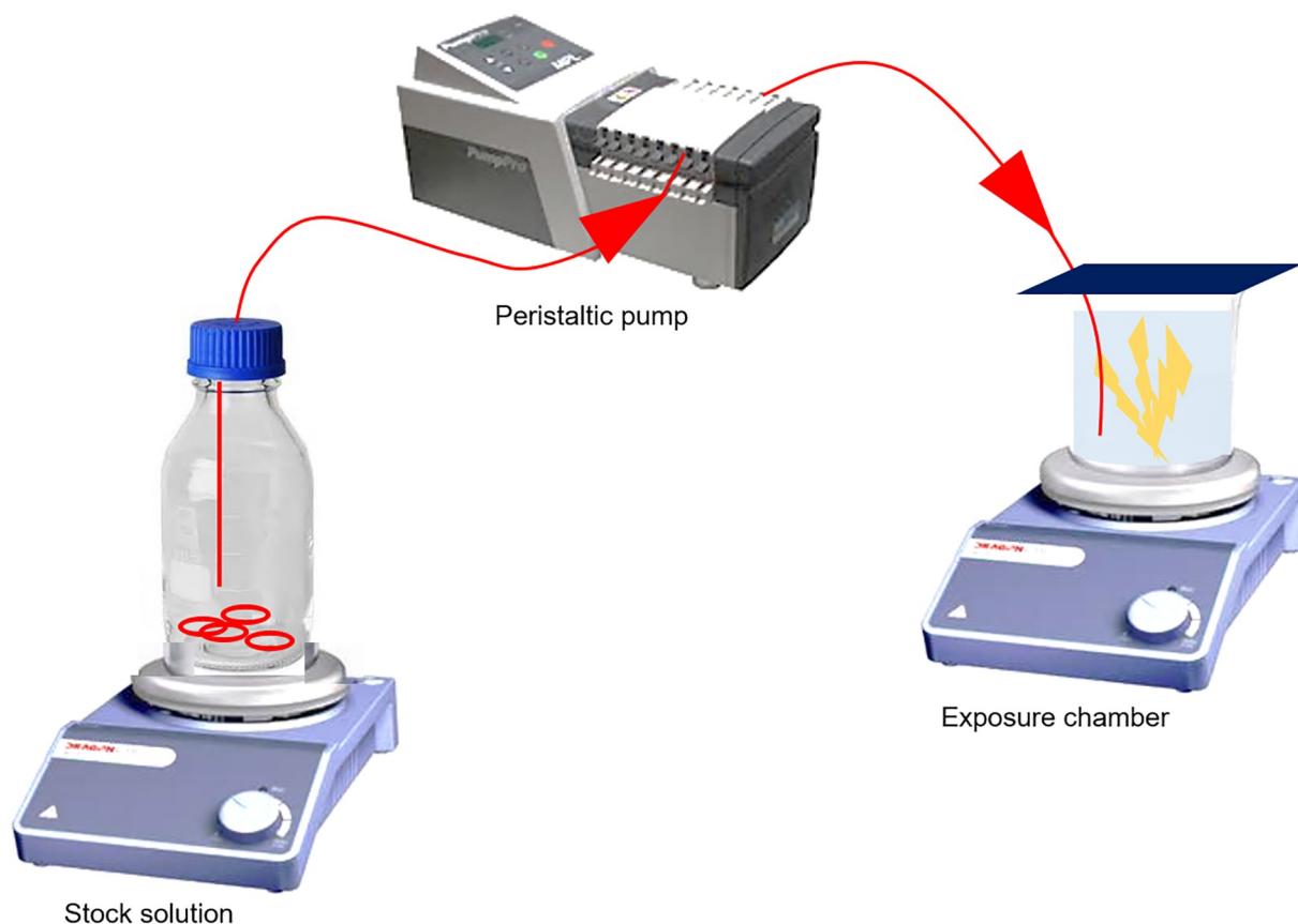
Fig 1. Setup for 2-methylnaphthalene exposure. Based on the principles of passive dosing described by Butler et al. [32], a passive dosage open system with flow-through using silicone O-rings has been developed. The peristaltic pump transfers stock solution from the stock bottle to the exposure chamber containing the test organisms.
