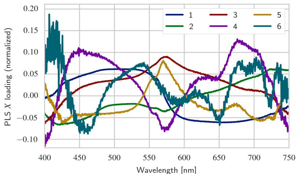
Fig 7. PLS X loadings for orange corals. Same as Fig 6, but created using data from orange corals. A notable difference is the significant noise in loading 6, indicating that explanatory power is decreasing at this point.
