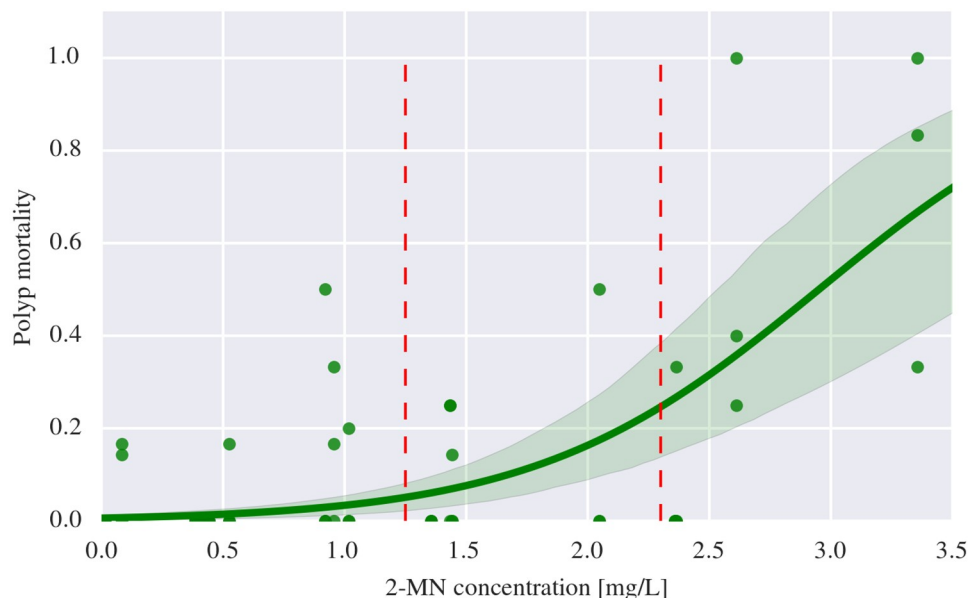
Fig 5. Dose-response curve for 2-methylnaphthalene exposure and polyp mortality ( n = 60 ). The regression line with a 95% confidence interval indicates that there is indeed a positive correlation between polyp mortality and 2-methylnaphthalene exposure. Some data points have similar values, and hence, overlap in the plot. The vertical red dashed lines indicate the 2-methylnaphthalene category thresholds and coincide with the 5% and 25% mortality levels (LC5 and LC25, respectively). The corresponding 2-methylnaphthalene concentrations are 1.25 \text{ mg L}^{-1} and 2.3 \text{ mg L}^{-1} , respectively.
