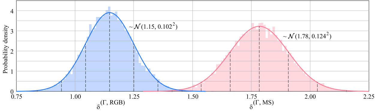
FIG. 5. Distributions of sample normalized spectral similarity \delta^{(\text{RGB}, \Gamma)} and \delta^{(\text{MS}, \Gamma)} between the polyp class and the skeleton class for the 10000 randomly selected samples of size 1000. The two distributions are approximately normal. By statistical inference, \delta^{(\text{MS}, \Gamma)} is larger than \delta^{(\text{RGB}, \Gamma)} in terms of 95% confidence intervals which implies that it is easier for the MS method to discriminate polyps from skeletons thanks to its finer-resolved spectrum than the RGB method.
