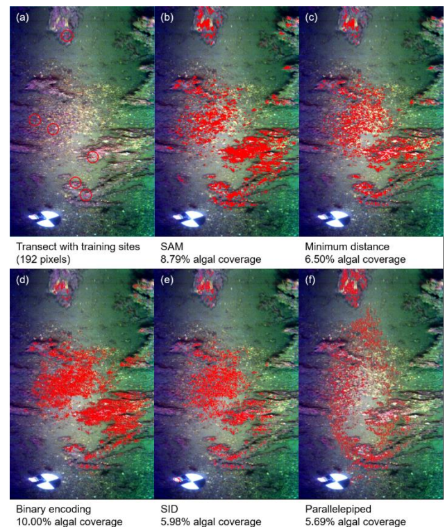
Fig. 10. Supervised classification of coralline algae in situ , based on upwelling radiance [ L_u(\lambda) ] from UHI-2. Classification was based on the mean L_u(\lambda) signature ( n = 192 pixels) of Phymatolithon tenue . Panel (a) shows the unclassified transect with training sites (32 pixels within each circle) highlighted in red. Panels (b-f) show the classification results of four different algorithms: spectral angle mapper [SAM; (b)], minimum distance (c), binary encoding (d), spectral information divergence [SID; (e)] and parallelepiped (f). Pixels classified as P. tenue are highlighted in red, and the estimated coralline algal coverage (%) from each algorithm is shown below its respective panel.
