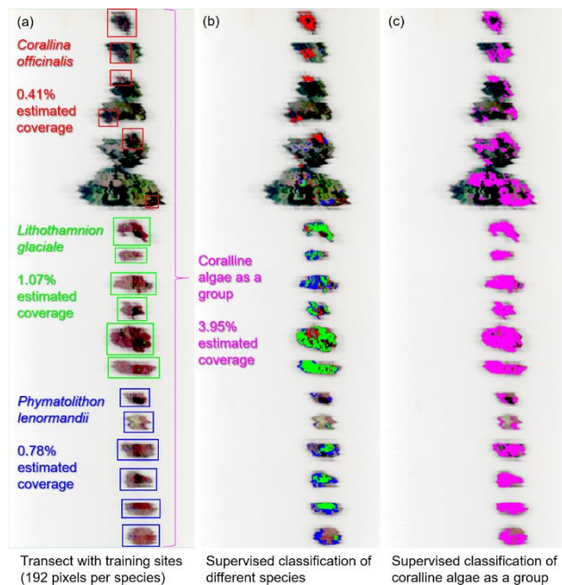
Fig. 9. Supervised classification of coralline algae in vivo , based on upwelling radiance [ L_u(\lambda) ] from UHI-1. The 2.00 x 0.60 m hyperspectral image transect was recorded in a scanning tank. Species classifications were based on the mean L_u(\lambda) signatures ( n = 192 pixels per species) of Corallina officinalis (red), Lithothamnion glaciale (green) and Phymatolithon lenormandii (blue). The group classification was based on the mean L_u(\lambda) signature ( n = 576 pixels) of all three species combined (pink). Panel (a) shows the unclassified transect with training sites indicated by small dots (16 pixels per dot) highlighted according to species. Panel (b) shows the results of spectral angle mapper classification of different coralline algal species. Classified pixels are colored according to species. Panel (c) shows the results of spectral angle mapper classification of coralline algae as a group. Pixels classified as coralline algae are highlighted in pink. Estimated transect coverage (%) is shown for each class.
