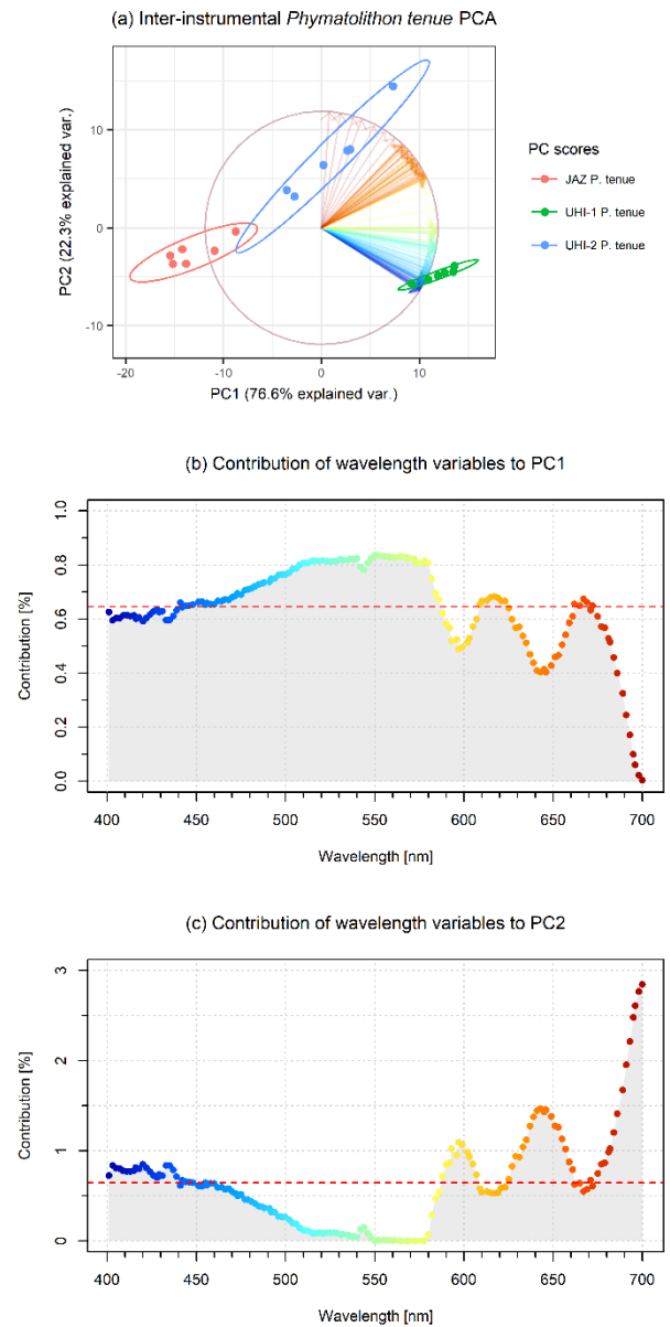
Fig. 7. Results of the principal component analysis (PCA) of inter-instrumental Phymatolithon tenue reflectance [ R(\lambda) ]. The analysis included R(\lambda) data from three different instruments: the JAZ spectrometer in vivo , UHI-1 in vivo and UHI-2 in situ ( n = 6 specimens per instrument). Panel (a) shows a biplot of the PCA results. Panels (b) and (c) show relative contributions (%) of the wavelength variables ( n = 155 ) to PCs 1 and 2. A comprehensive description of the figure elements is presented in the Fig. 6 caption.
