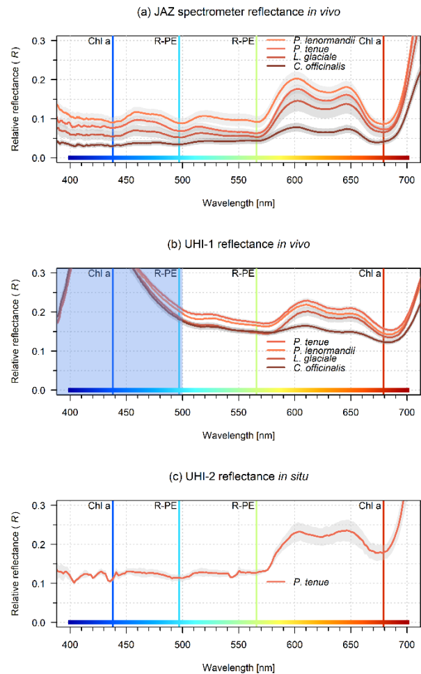
Fig. 5. Mean JAZ spectrometer (a), UHI-1 (b) and UHI-2 (c) reflectance [ R(\lambda) ] spectra ( n = 6 ) of four coralline algal species: Corallina officinalis , Lithothamnion glaciale , Phymatolithon lenormandii and Phymatolithon tenue . JAZ spectrometer and UHI-1 R(\lambda) spectra were obtained in vivo , and included all four species. UHI-2 R(\lambda) spectra were obtained in situ , and only included P. tenue . Gray shaded areas represent the R(\lambda) spectra's associated 95% confidence intervals. Vertical lines represent in vivo absorbance maxima of the pigments chlorophyll a (Chl a) [9, 10] and R-phycoerythrin (R-PE) [15–17]. The blue shaded area in panel (b) represents wavelengths where R(\lambda) estimates from UHI-1 are considered to be overestimated (i.e. erroneous).
