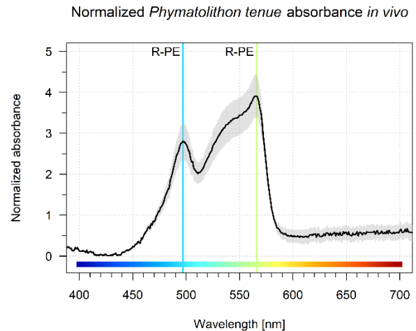
Fig. 3. Mean in vivo normalized absorbance spectrum ( n = 6 ) of the coralline algal species Phymatolithon tenue . The gray shaded area represents the associated 95% confidence interval. Vertical lines represent in vivo absorbance maxima of the pigment R-phycoerythrin (R-PE) [15-17].
