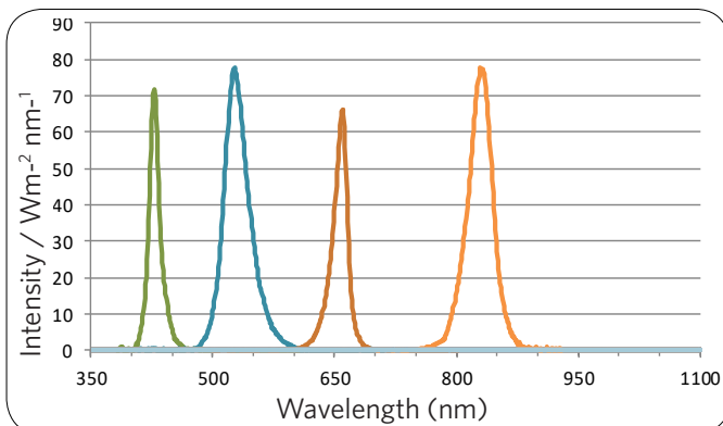
Spectral Characteristics -RGB-IR
