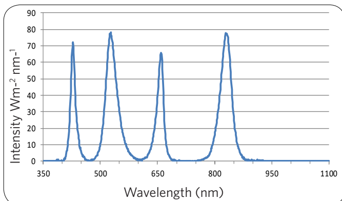
Intensity vs Wavelength -RGB-IR
