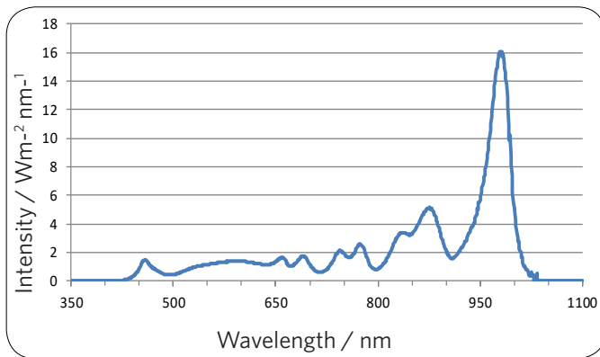
Intensity vs Wavelength - 8 wavelength
