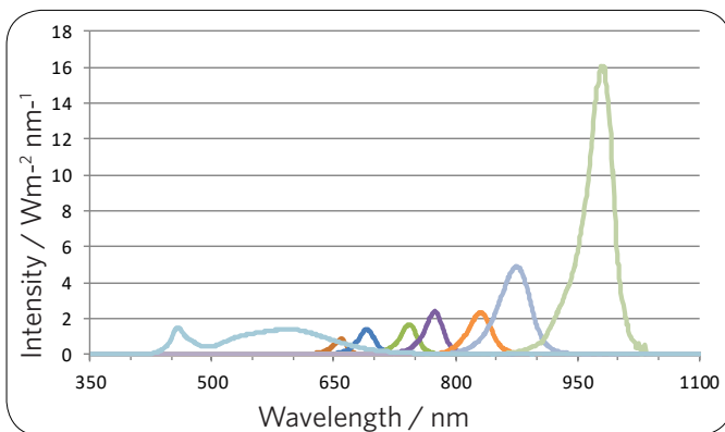
Spectral Characteristics - 8 wavelength
