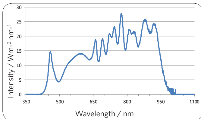
Intensity vs Wavelength - 10 wavelength
