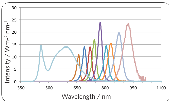
Spectral Characteristics - 10 wavelength
