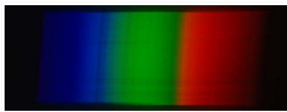
— Figure 6: Solar spectrum (through slit) captured with the same camera and grating as the other photographs. Not much yellow or cyan to be seen, reflecting sharp filter cutoffs. Absorption lines (Fraunhofer lines) are visible in the spectrum, arising from constituents in the solar atmosphere.
