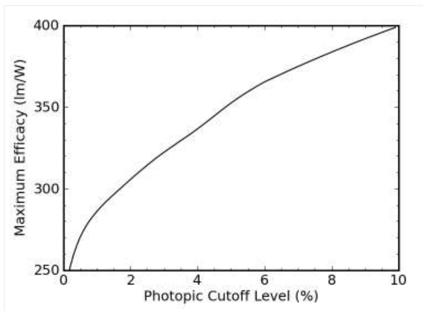
— Figure 9: Luminous efficacy achievable with truncated blackbody, as a function of truncation degree.
