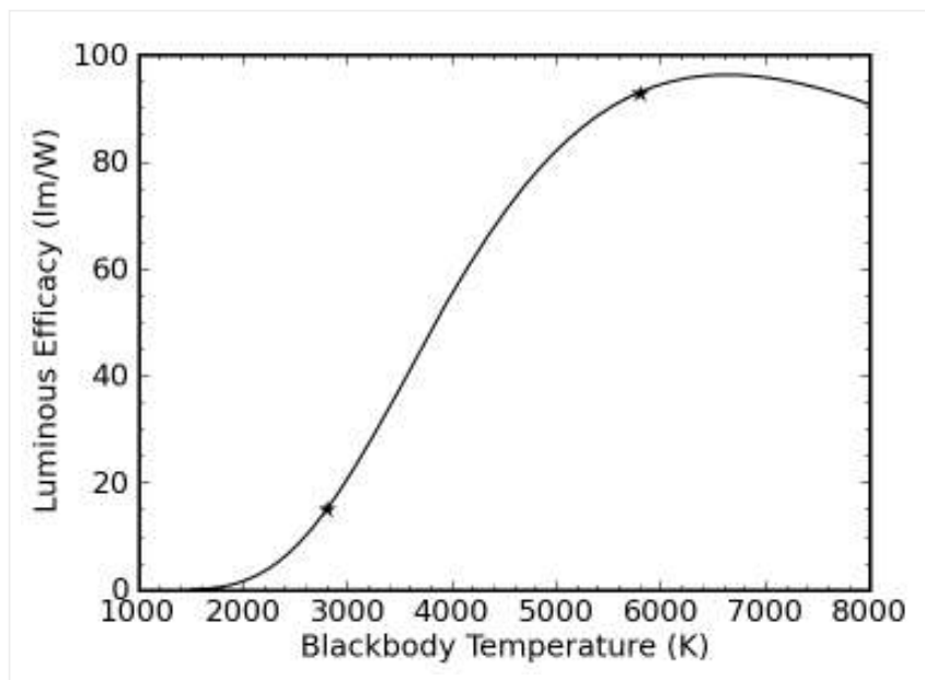
— Figure 8: Luminous efficacy of pure blackbody sources.
