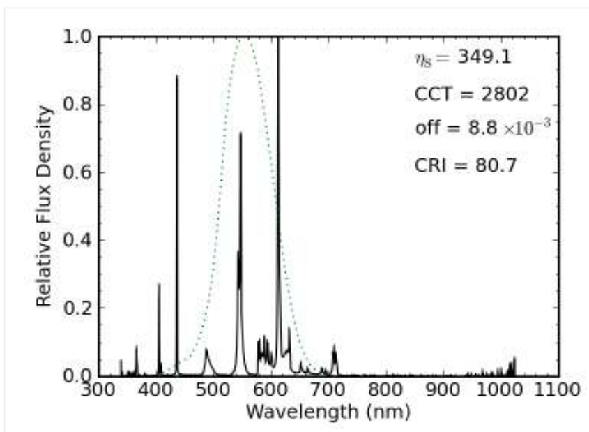
— Figure 13: Same CFL bulb after warming up. Some semi-broad phosphors are used for continuum light, but lines still dominate.
