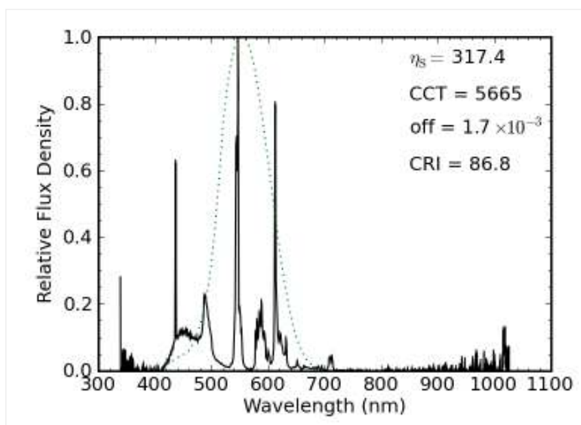
— Figure 16: Laptop screen illuminated by fluorescent light. Still line dominated, although the phosphors are broader than those used in the CFL bulb.
