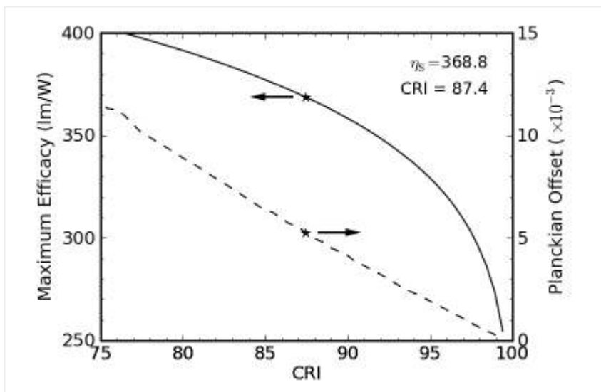
— Figure 11: Maximum performance of a truncated 2800 K blackbody as a function of allowable color rendering performance.
