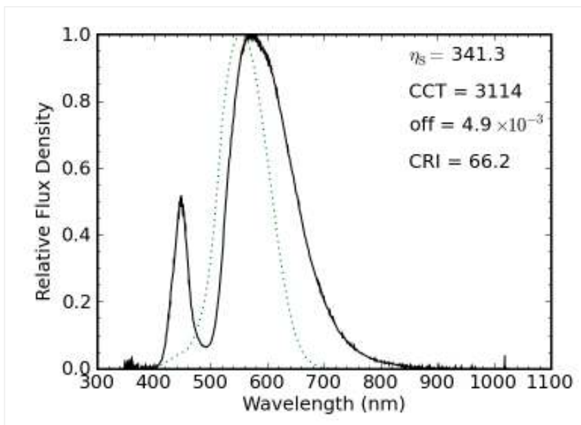
— Figure 14: A "warm" LED light spectrum. One blue LED pumps a broad-band yellow phosphor.
