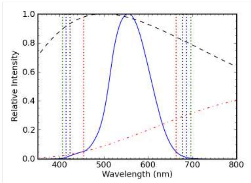
— Figure 7: The photopic sensitivity curve (blue) compared to the solar blackbody spectrum (black) and a blackbody at a temperature characteristic of incandescent bulbs (red).
