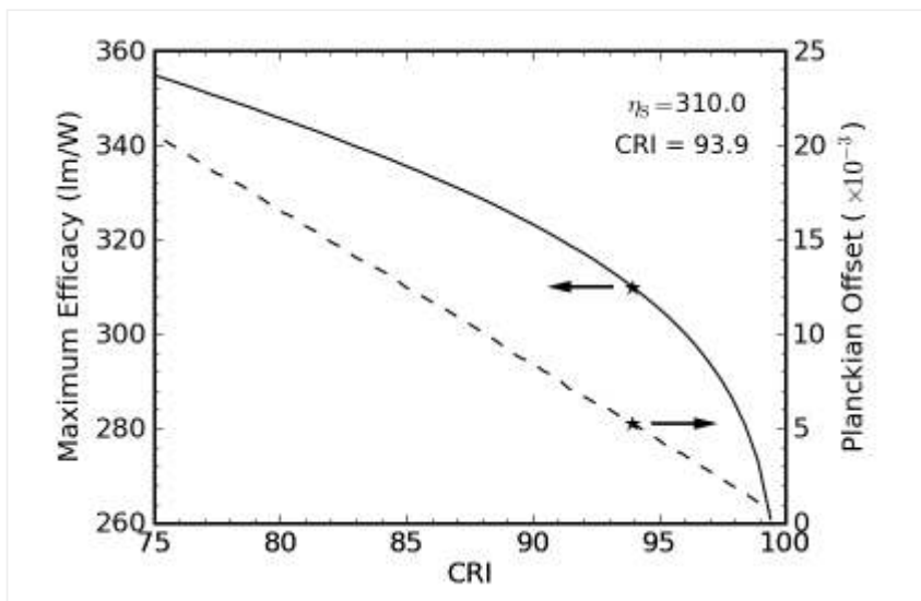
— Figure 10: Maximum performance of a truncated 5800 K blackbody as a function of allowable color rendering performance.
