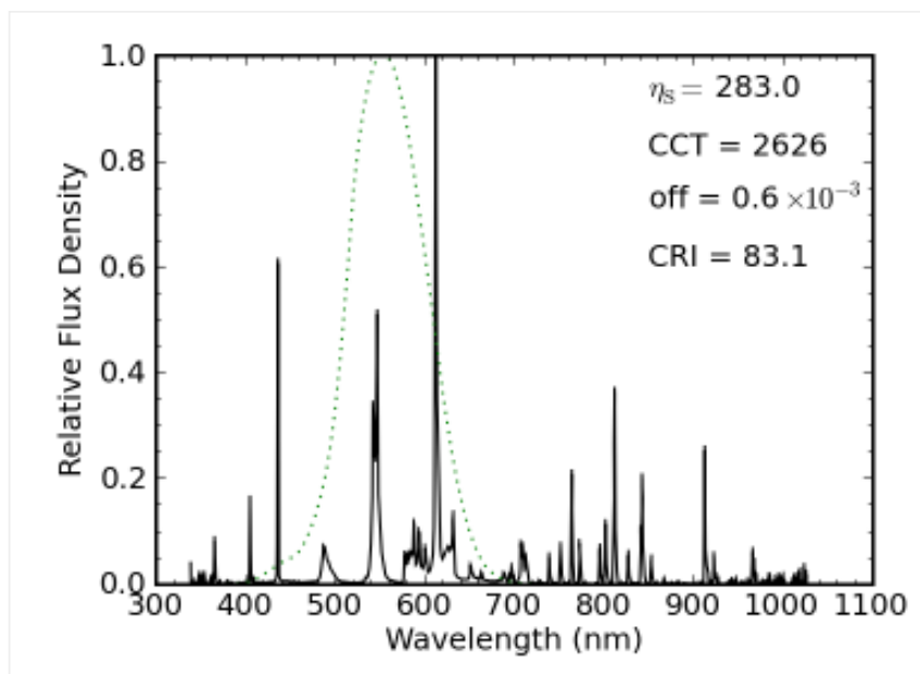
— Figure 12: A compact fluorescent light (CFL) seconds after being turned on. The spectrum is dominated by line sources, with a forest of infrared lines that will later disappear.
