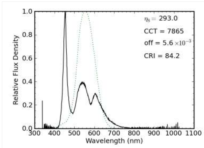
— Figure 17: Laptop screen illuminated by LED lighting. Same concept: blue LED pumps phosphors—in this case a green and a red.
