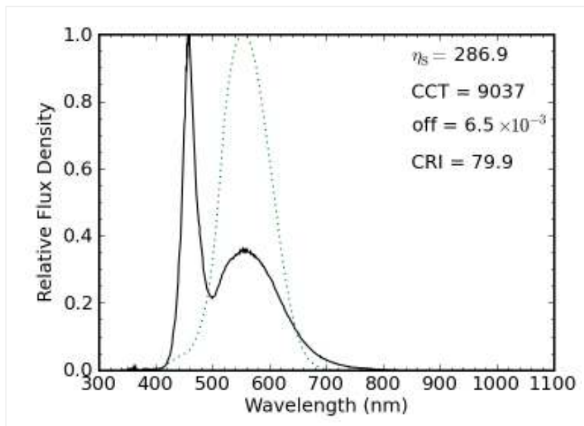
— Figure 15: Similar to the bulb before, this LED light uses a blue LED to pump a broad-band phosphor, but less so.
