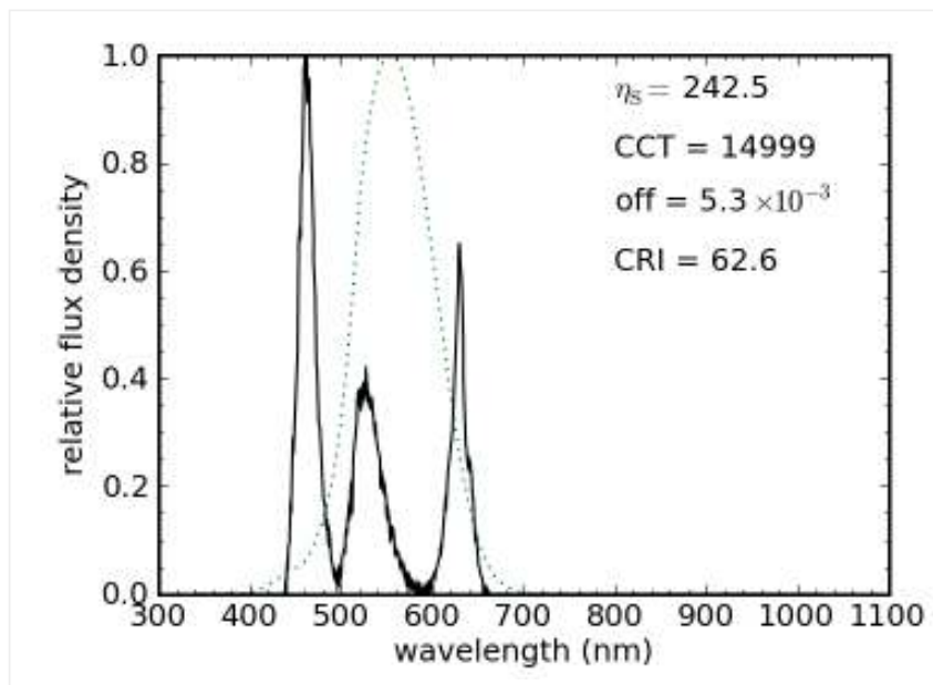
— Figure 19: Three-LED (blue, green, red) mixture giving a white-ish light.
