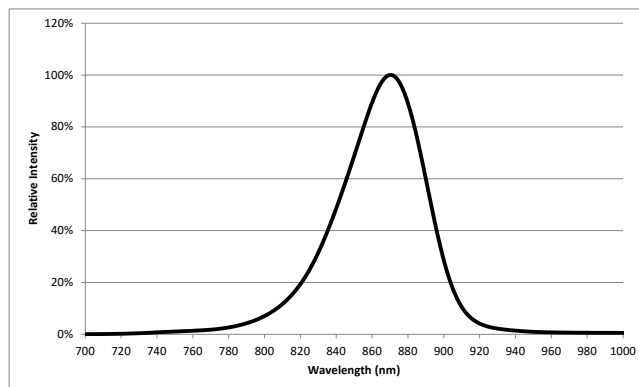
Typical Spectra
