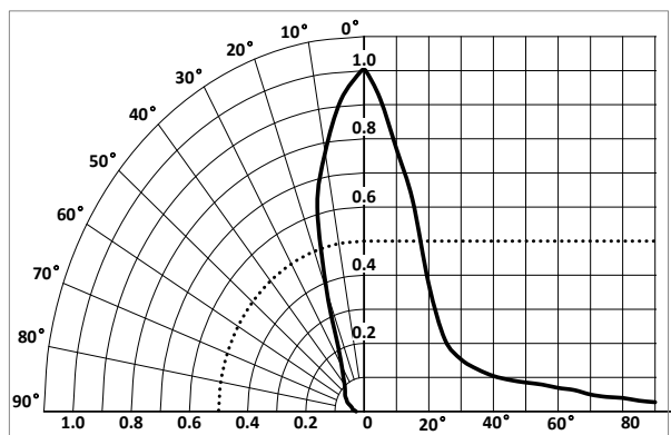
Typical Polar Radiation Plot - B40
