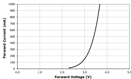
FIGURE 10 ELECTRICAL CHARACTERISTICS OF XR-E LED (TJ = 25 °C)
