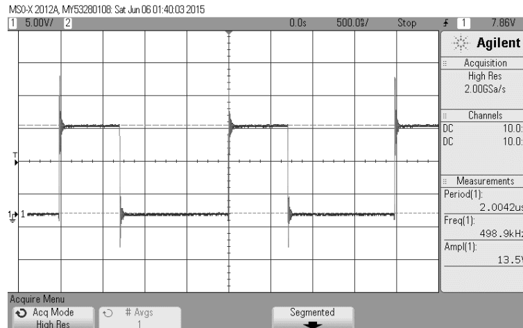
FIGURE 52 DRAIN VOLTAGE OF Q1
