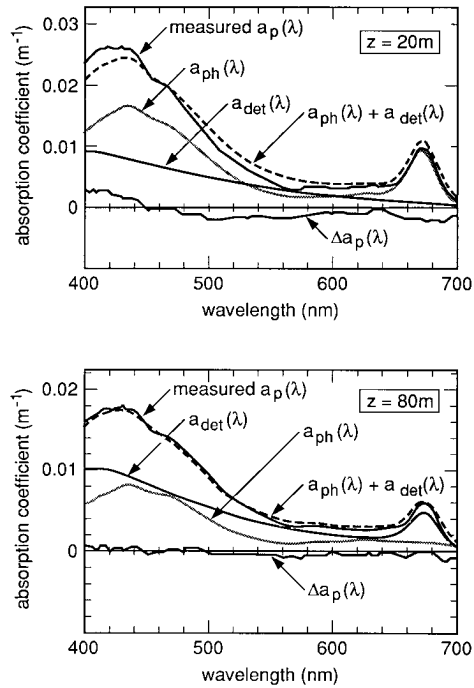
FIGURE 8 Examples of the relative contributions of absorption by phytoplankton a_{ph}(\lambda) , and by organic detritus a_{det}(\lambda) , to the total particulate absorption a_p(\lambda) , from Sargasso Sea waters. (Redrawn from Iturriaga and Siegel, 46 with permission.)
