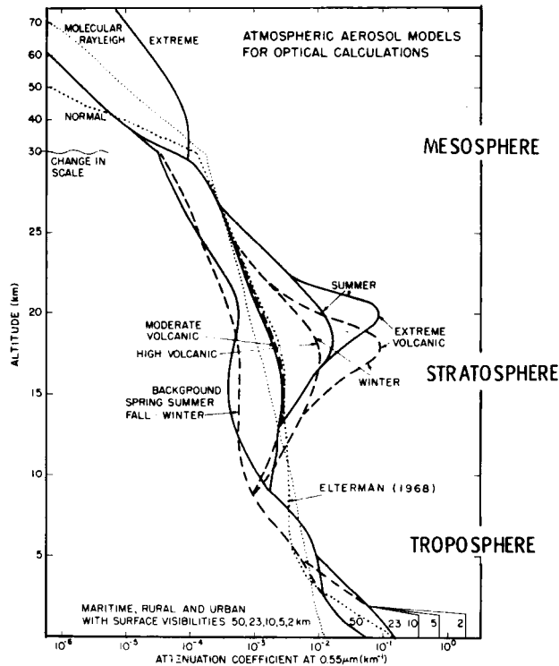
FIGURE 17 The vertical distribution of the aerosol extinction coefficient (at 0.55\text{-}\mu\text{m} wavelength) for the different atmospheric models. Also shown for comparison are the Rayleigh profile (dotted line). Between 2 and 30 km, where the distinction on a seasonal basis is made, the spring-summer conditions are indicated with a solid line and fall-winter conditions are indicated by a dashed line. (From Ref. 3.)
