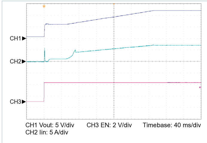
Figure 15 — Startup from EN, V_{IN} = 48\text{ V} , C_{OUT\_EXT} = 10000\text{ }\mu\text{F} , R_{LOAD} = 0.450\text{ }\Omega
