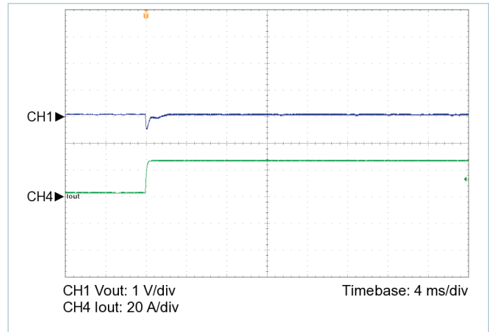
Figure 6 — 10% to 100% load transient response, V_{IN} = 48\text{ V} , nominal trim, C_{OUT\_EXT} = 1000\text{ }\mu\text{F}
