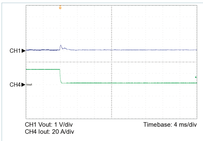
Figure 5 — 100% to 10% load transient response, V_{IN} = 48\text{ V} , nominal trim, C_{OUT\_EXT} = 1000\text{ }\mu\text{F}
