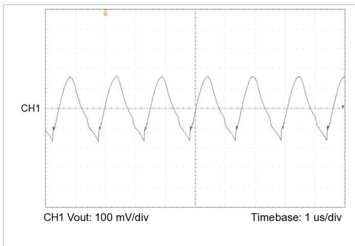
Figure 17 — Output voltage ripple, V_{IN} = 48\text{ V} , V_{OUT} = 12.0\text{ V} , C_{OUT\_EXT} = 1000\text{ }\mu\text{F} , R_{LOAD} = 0.450\text{ }\Omega
