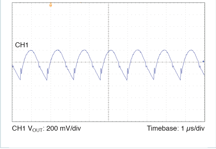
Figure 16 — Output voltage ripple, V_{IN} = 270\text{ V} , V_{OUT} = 12.0\text{ V} , C_{OUT\_EXT} = 1000\text{ }\mu\text{F} , R_{LOAD} = 0.288\text{ }\Omega
