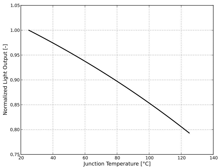
Figure 2d. Typical normalized radiant power vs. junction temperature for LUXEON 2835 White at 120mA.
