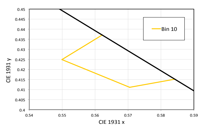
Figure 7. Color Bin Structure for LUXEON 2835 PC Amber for Table 9.
