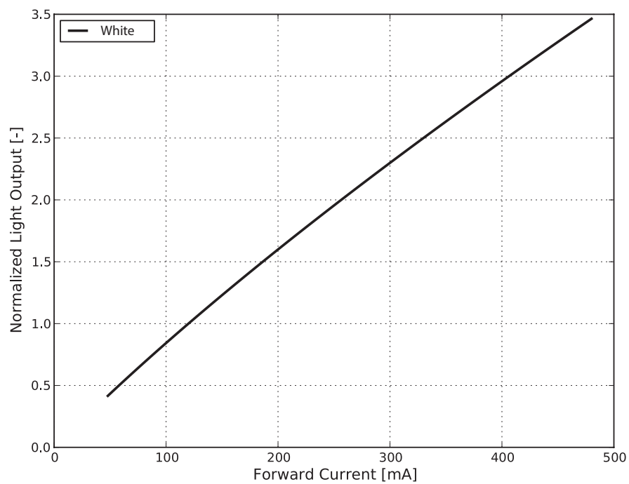
Figure 3d. Typical normalized radiant power vs. forward current for LUXEON 2835 White at T_j=25^{\circ}\text{C} .
