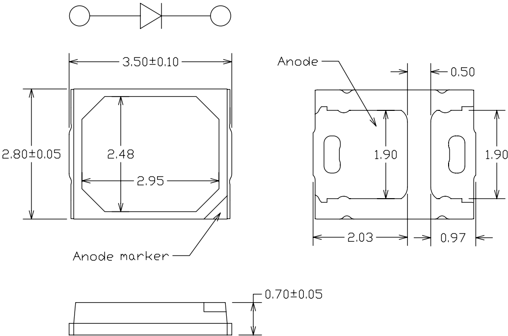
Figure 11. Mechanical dimensions for LUXEON 2835 Color Line.
