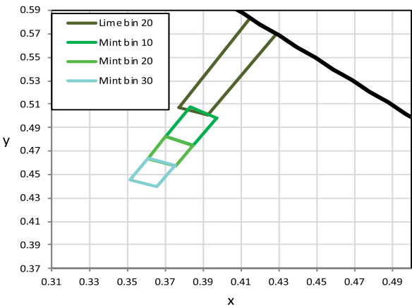
Figure 8. Color Bin Structure for LUXEON 2835 Lime and Mint for Table 9.
