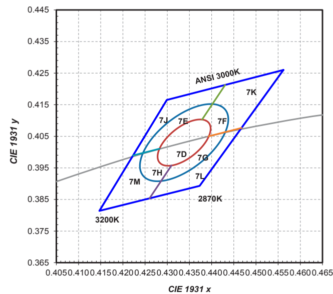
Figure 10a. 1/9 th color bin structure for LUXEON 2835 White 3000K at test current and binning temperature of T j =25°C.
