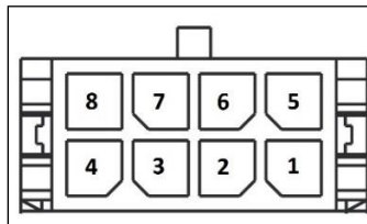
Figure 4-5: Molex Micro-fit P/N 43045-0800
