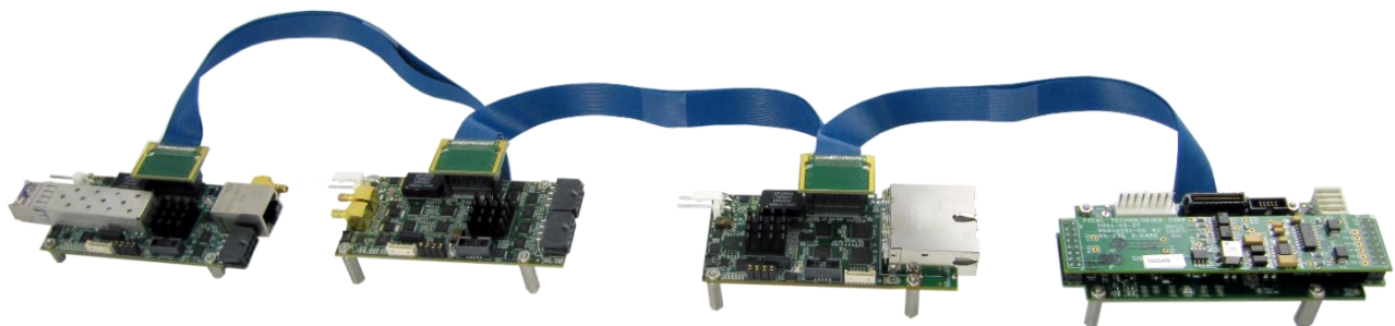
Figure 1-3: 914-X Series System with Tethered Expansion Cards
