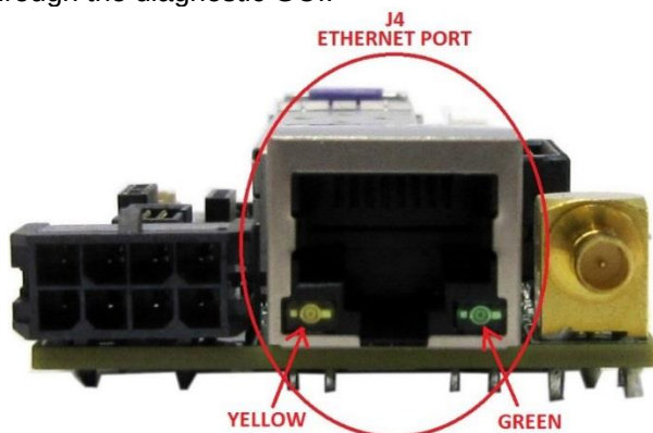
Figure 4-7: Ethernet Port
