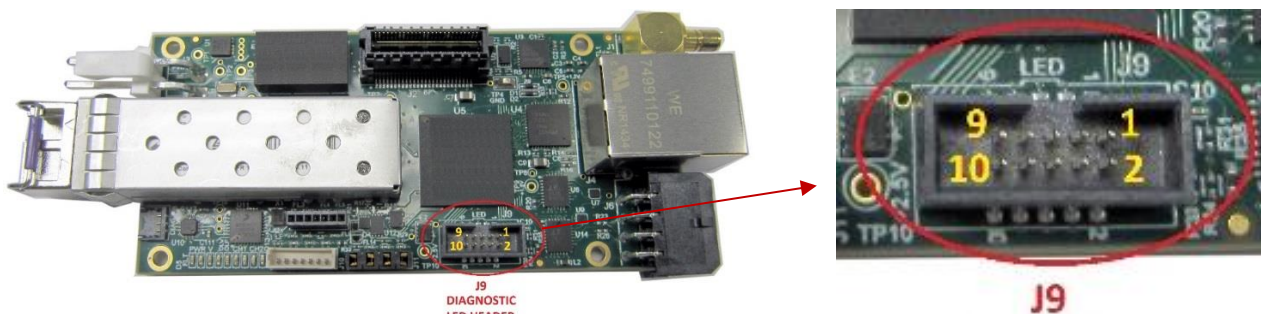
Figure 4-10: Diagnostic LED Header
