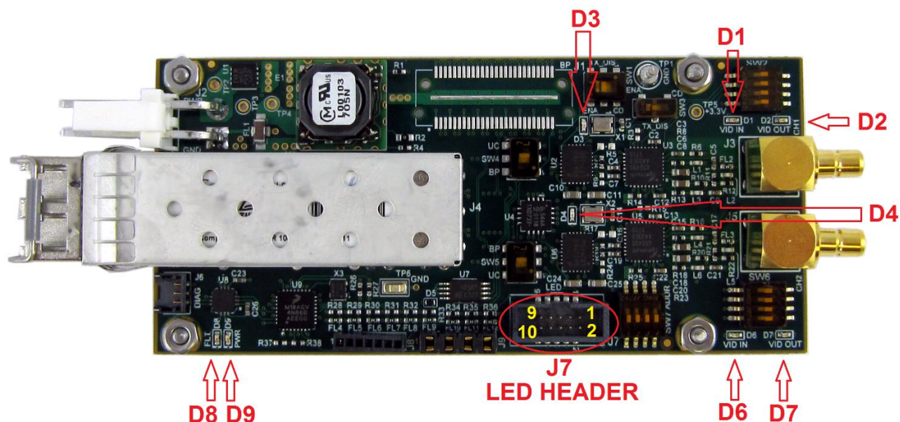
Figure 7-8: 914-HDV2 Diagnostic LEDs and LED Header
