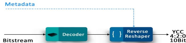
Figure 8-4 HDR Decoding Process
