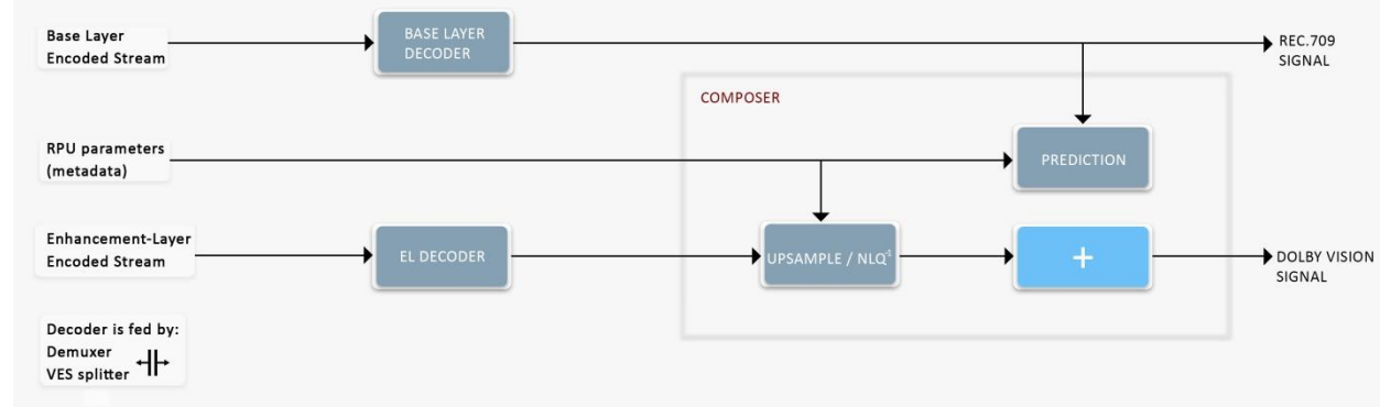
Figure 9-7 Composer - Dolby Vision (Source: Dolby)
