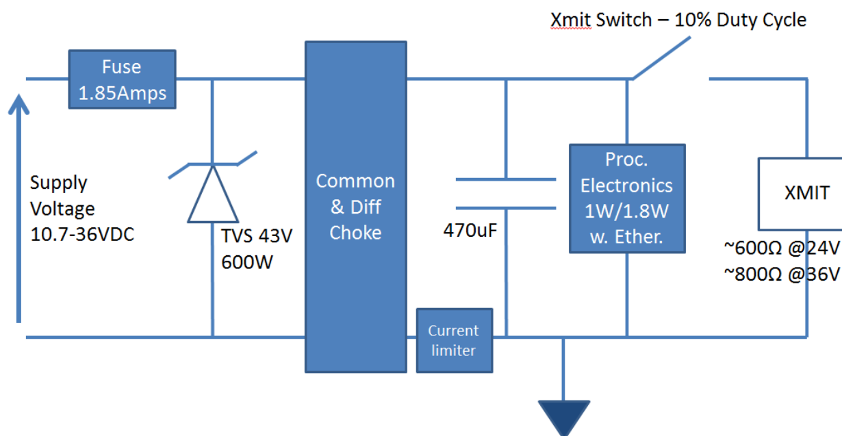
Figure 23. Pathfinder Power Circuit
