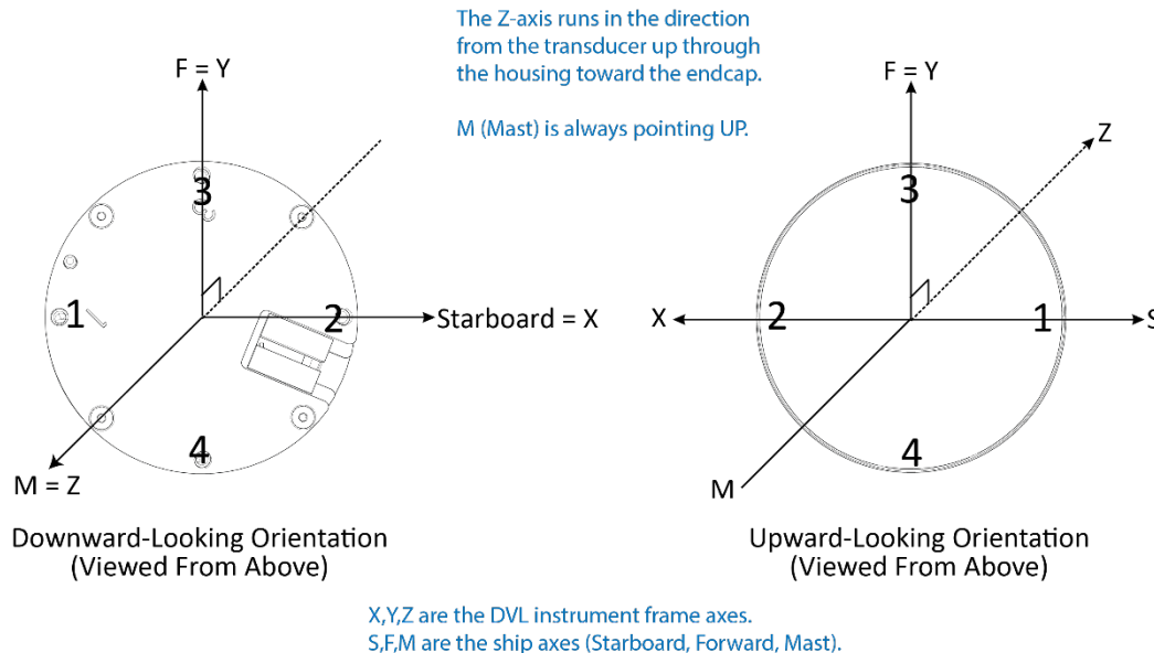
Figure 17. Pathfinder Ship Coordinates (OEM Transducer Shown)
