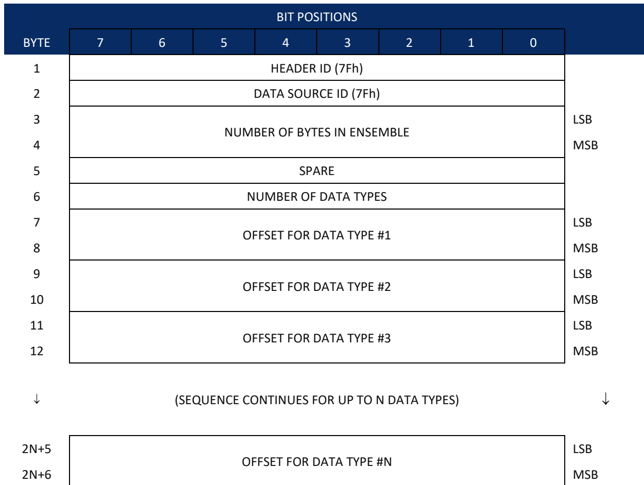
Figure 30. Binary Header Data Format
