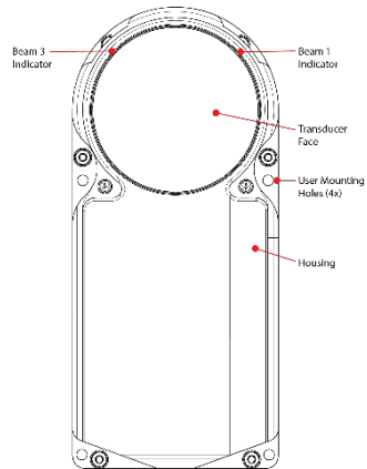
Figure 24. Transducer View
