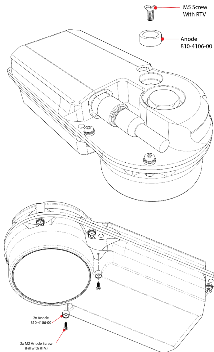
Figure 26. Replacing an Anode
