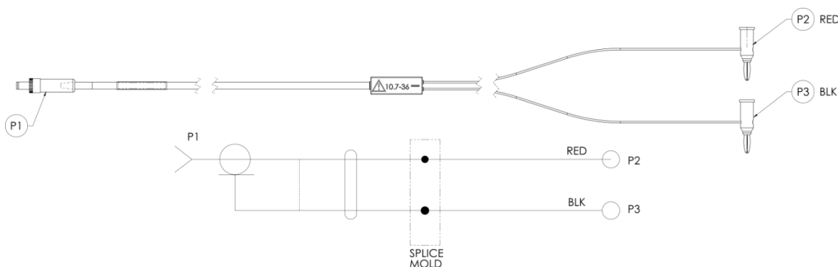
Figure 9. Power Adapter Cable 73B-6046-00
