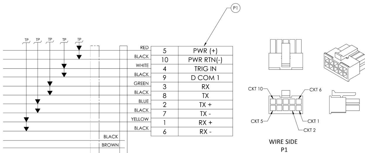
Figure 11. Pathfinder OEM Power/Comm Cable 73B-6060 Pigtail Cable
