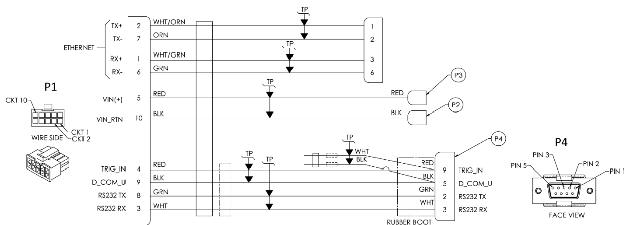
Figure 7. OEM Pathfinder Connections for Bench Test [73B-6059-00 Cable]
