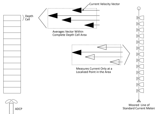
Figure 15. DVL Depth Cells for Current Measurements
