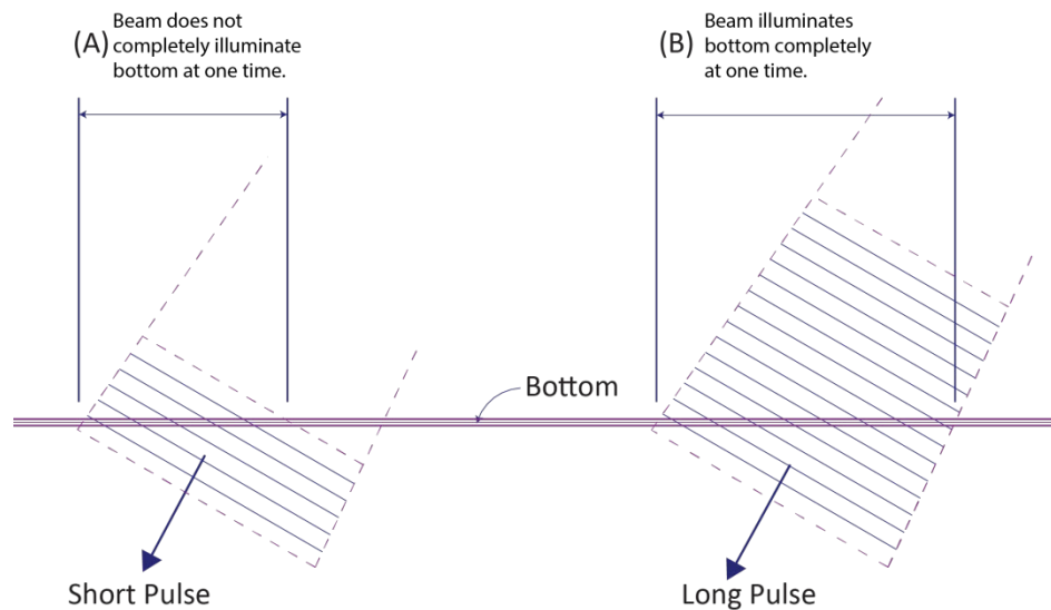
Figure 13. Short Pulse versus Long Pulse
