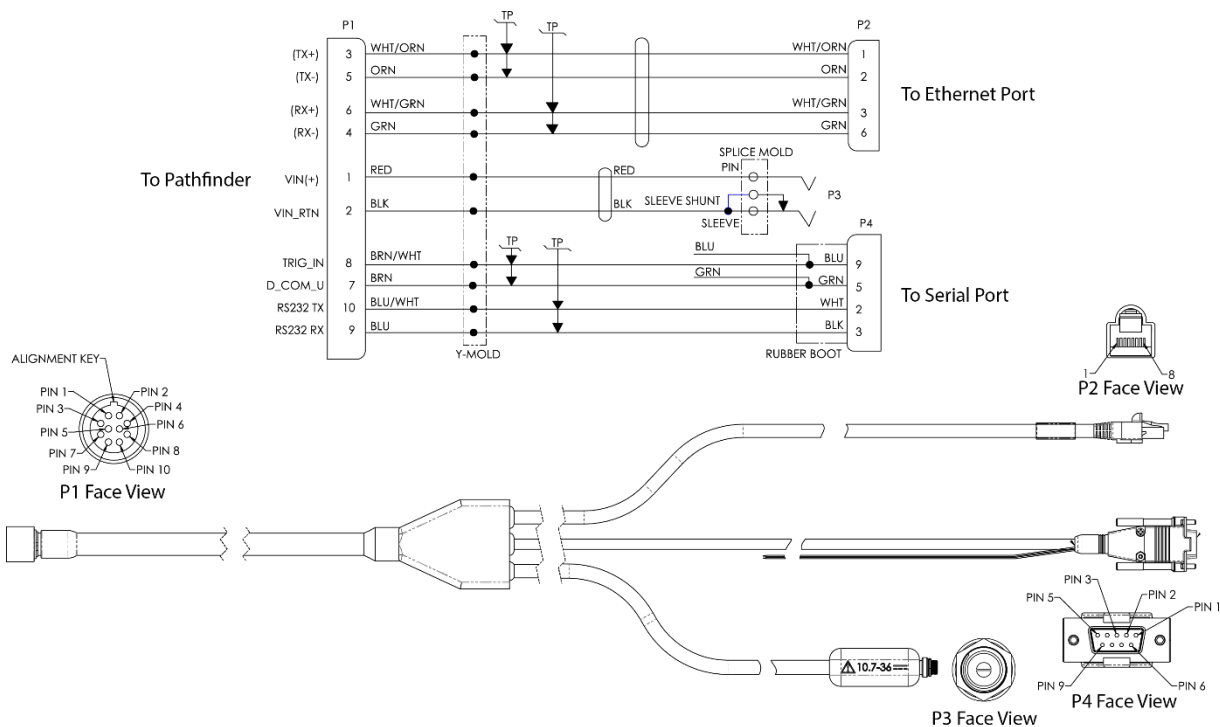
Figure 8. Pathfinder Power/Comm Cable 73B-6057-005 Optional Test Cable
