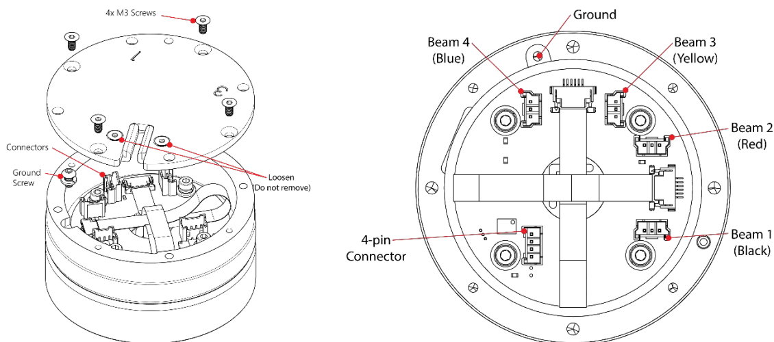
Figure 6. OEM Pathfinder Transducer Connections
