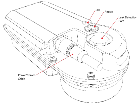
Figure 25. Top View
