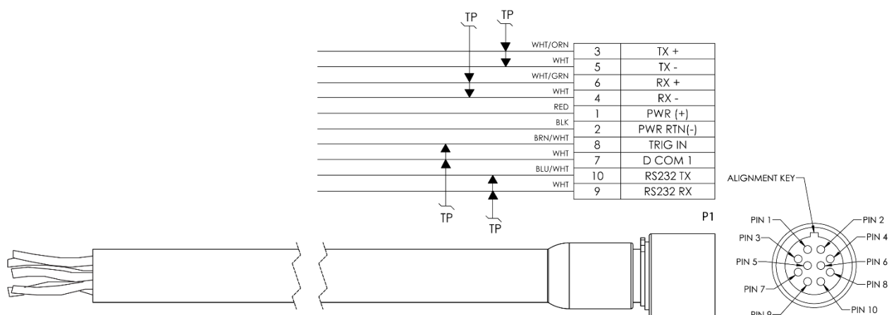
Figure 10. Pathfinder ROV Power/Comm Cable 73B-6058 Pigtail Cable
