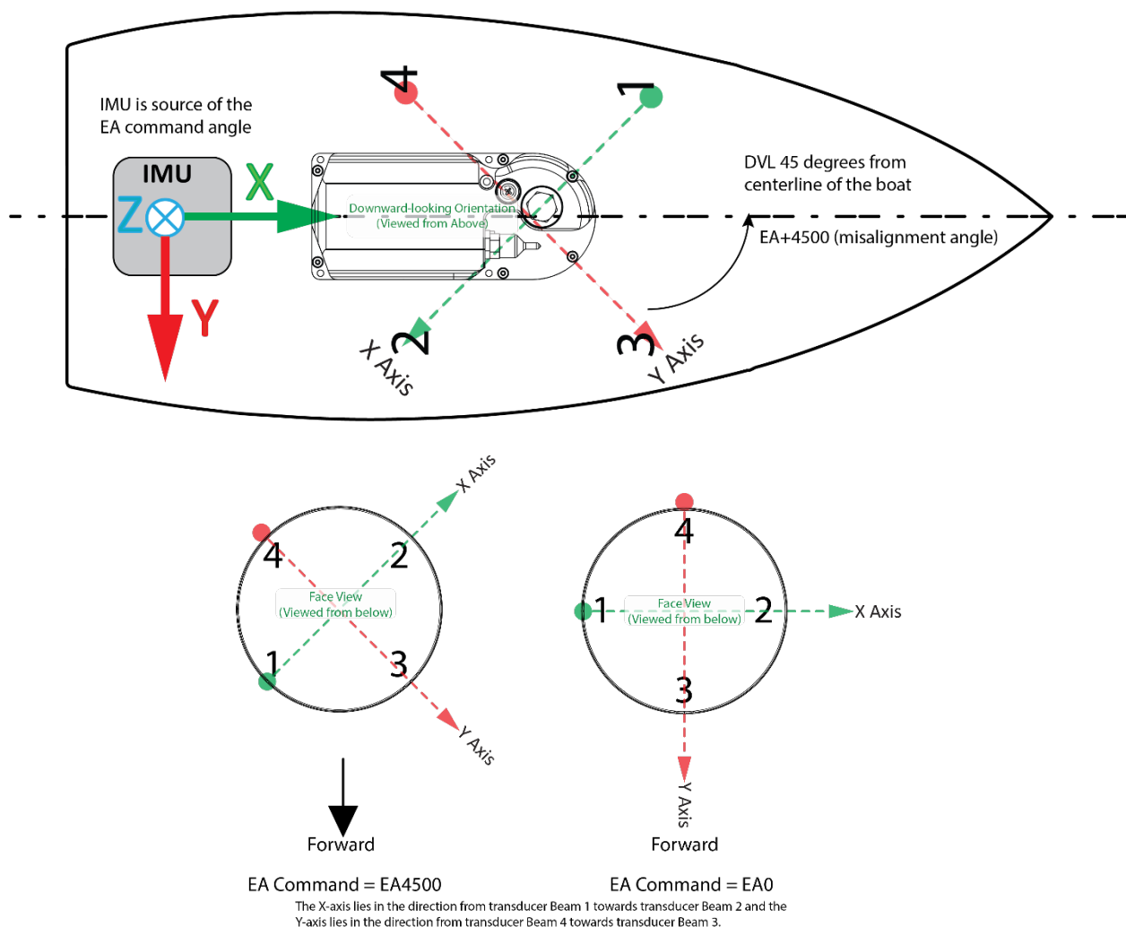
Figure 19. Transducer Alignment Reference Points
