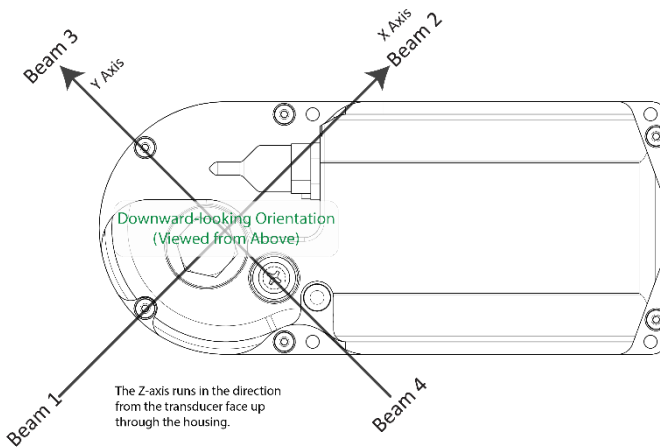
Figure 16. X, Y, and Z Velocities (ROV version shown)
