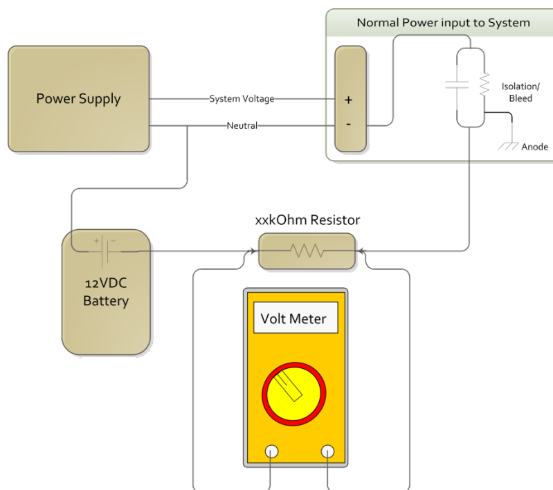
Figure 22. Ground Fault Current Check
