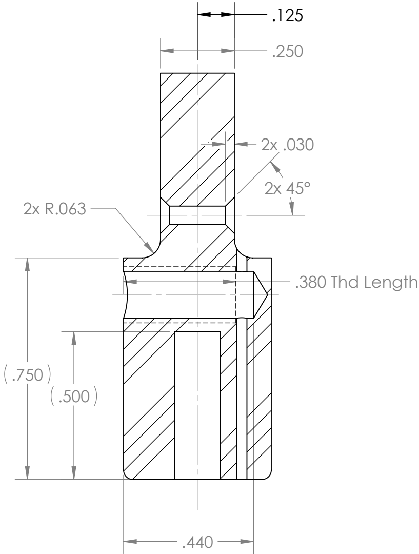
SECTION F-F SCALE 3 : 1
