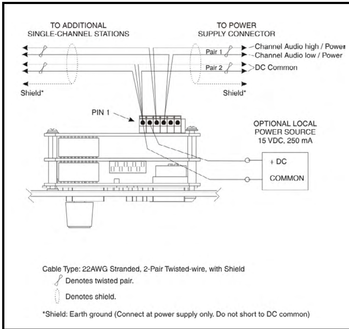
FIGURE 6. Audiocom mode connections for WM1000 Intercom Station.
