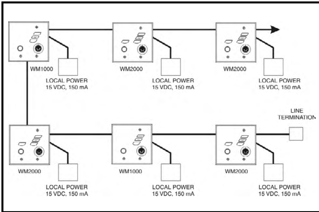
FIGURE 5. Locally powered intercom system
