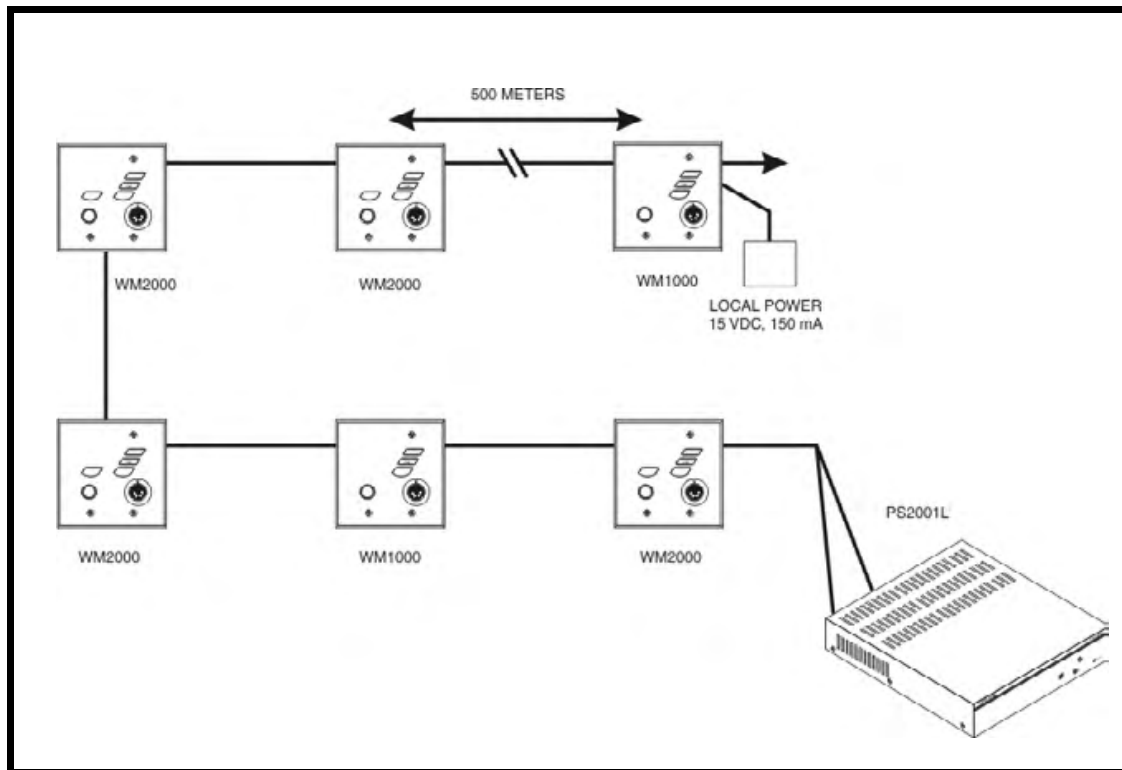
FIGURE 2. PS2001L Power Supply set to isolate mode
