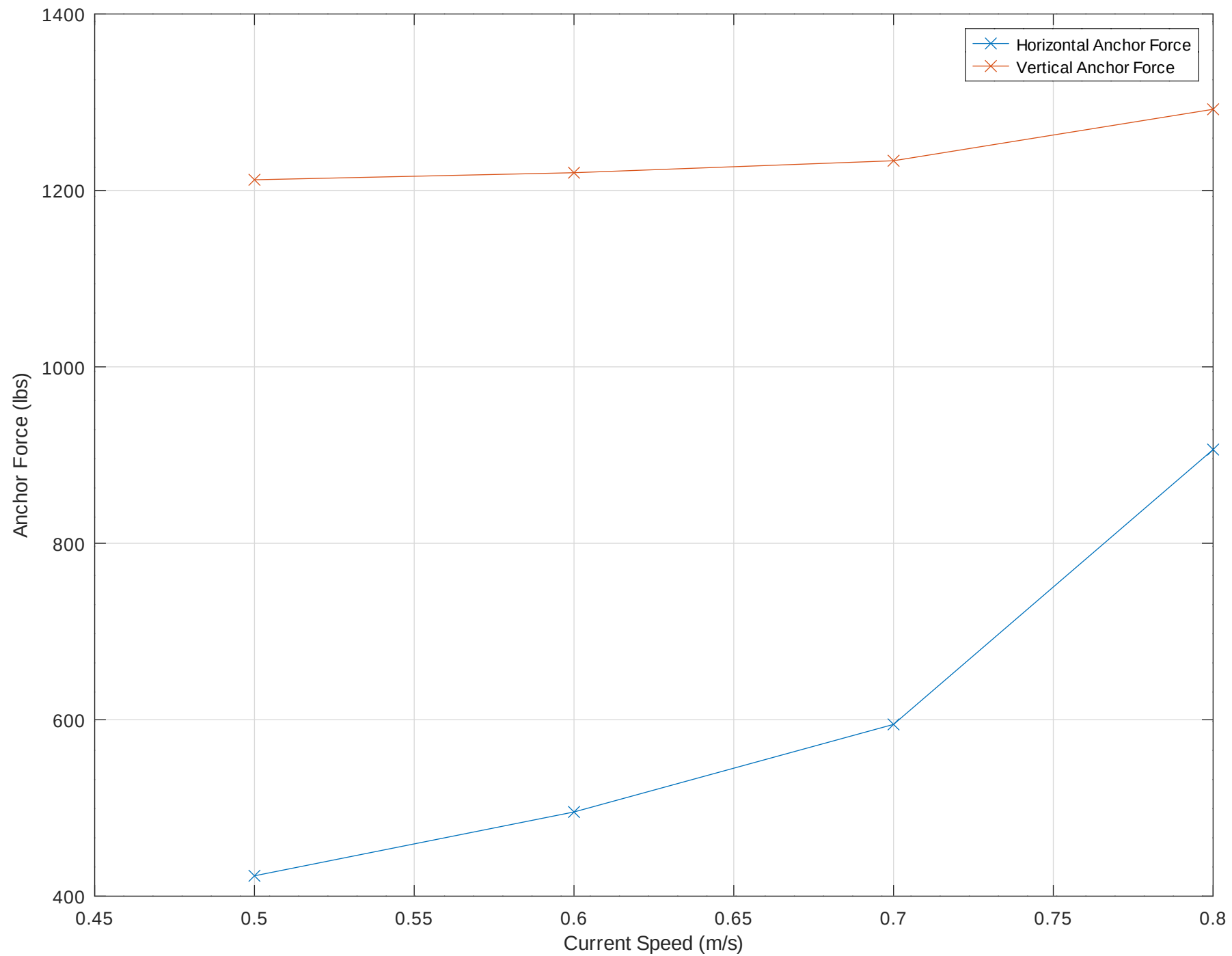
Anchor Loads in Static Conditions: Depth = 52m Wind = 0kts
