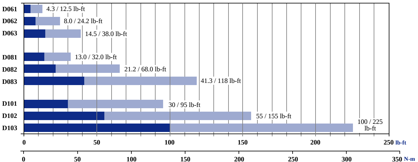
Peak and Continuous Torque by Model
