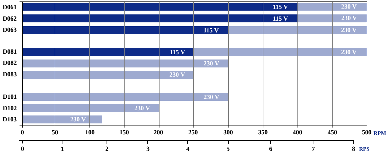
Maximum Speed by Model
