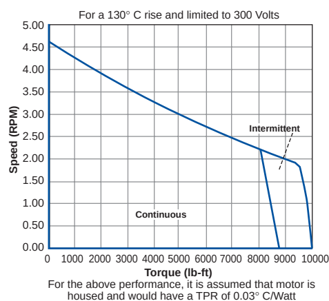
Continuous Operation Curve
