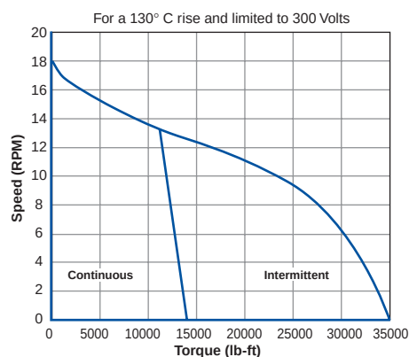
Continuous Operation Curve
