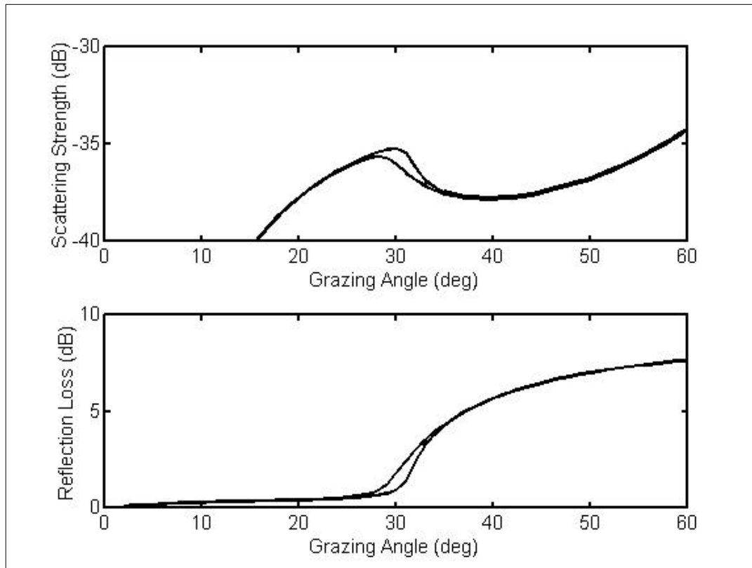
Figure 6. The predicted extremes of the seasonally dependent seafloor backscattering strength and reflection loss at 1 kHz with diffusivity 0.0014 \text{ cm}^2\text{s}^{-1} .
