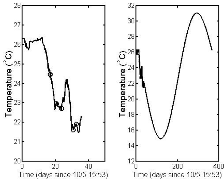
Figure 2. The left panel displays water temperature at the seafloor obtained during the SAX99 experiment. The symbols “o” mark the times at which sediment temperature profile data were taken. The right panel displays a temperature time series spanning one year in which the measured data were supplemented by a simple fit to data from [4].
