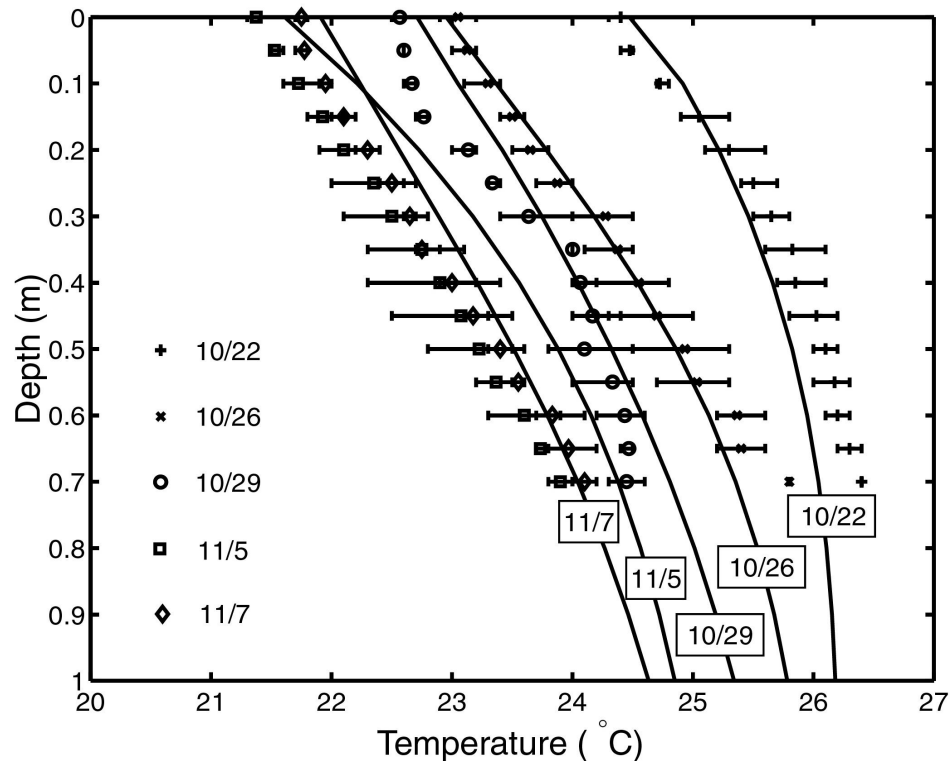
Figure 5. Comparison of sediment temperature profile data (mean values, with extremes shown as error bars) with the heat conduction model. The five model curves and the corresponding symbols used for measurements are labelled with the measurement date.
