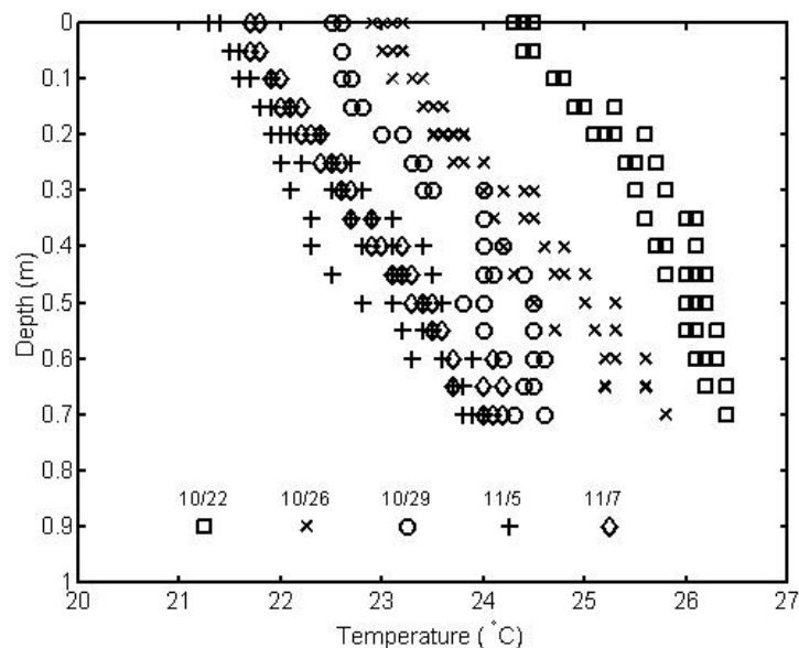
Figure 3. Sediment temperature profile data obtained during SAX99 experiment. Each symbol corresponds to the given date, for which there were three or more temperature probe insertions. Temperature values at the sediment surface are in agreement with the near-bottom water column temperature of Figures 1 and 2.
