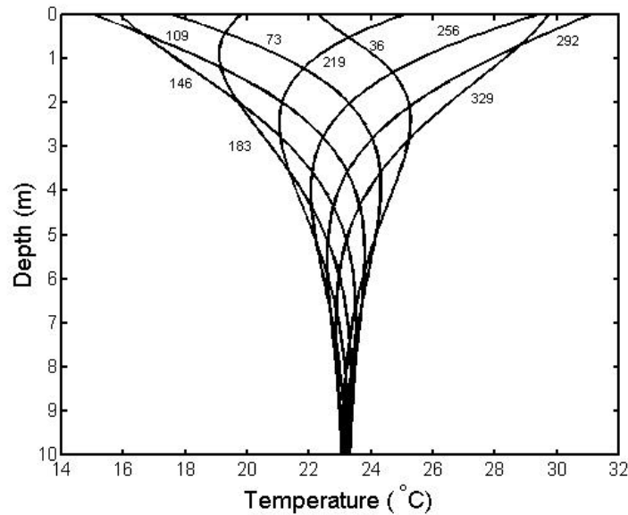
Figure 4. Synthetic temperature profiles obtained by solving the one-dimensional heat diffusion equation with diffusivity 0.006 \text{ cm}^2\text{s}^{-1} . The curves are labelled by the time (in days) from the beginning of the water temperature time series of Figure 2.
