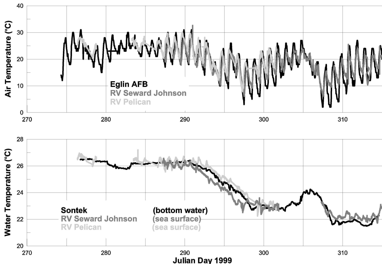
Figure 1. Air, surface, and bottom water temperatures measured during the SAX99 experiment (1 October through 11 November 1999 or Julian dates 274 to 315 in the figures). The start of a given Julian day was chosen to coincide with 0000 hours, local daylight time). Air temperatures were measured at Eglin AFB (16 km northeast of the study site) and from the two research vessels while operating in the vicinity of the SAX99 experiment. Water
