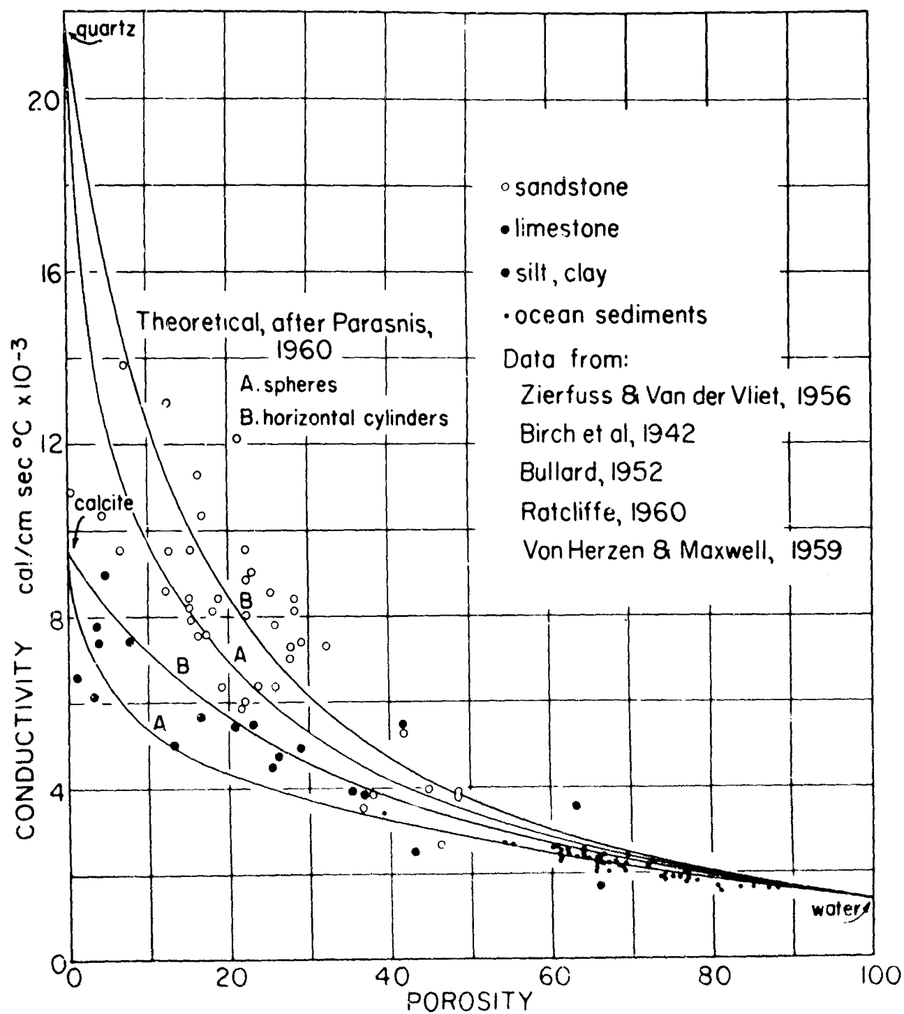
Figure 6 Thermal conductivity-porosity data for ocean sediments, sandstones and limestones compared with theoretical curves adapted from Parasnis (1960).
