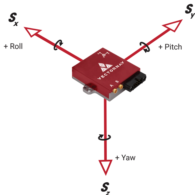
(a) Sensor-Frame
