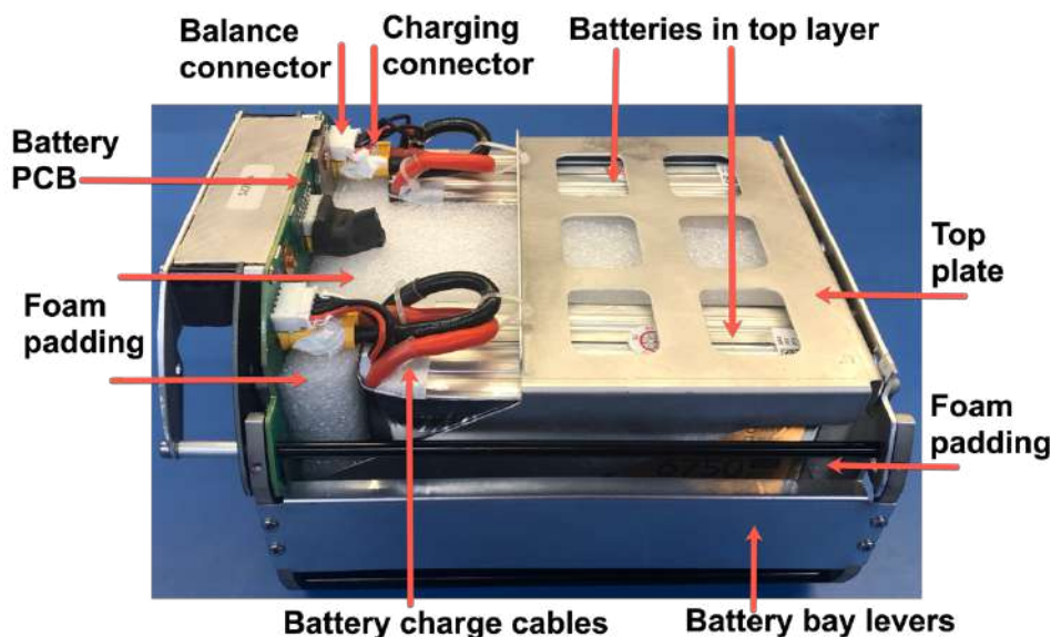
Battery pack for Boxfish Alpha
