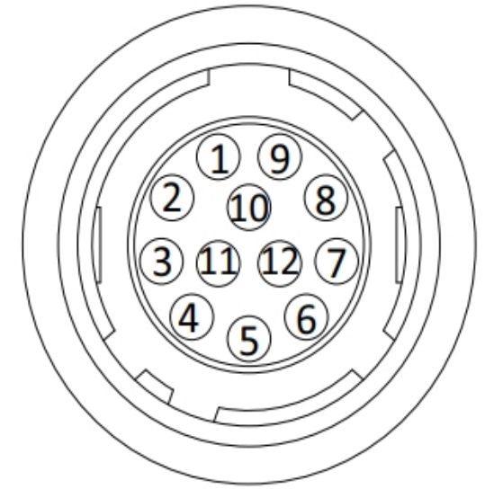
Receptical View (mirror of plug)
